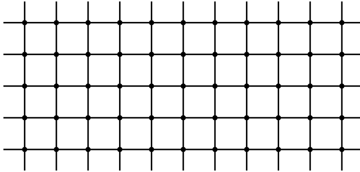
Figure 6: Part of the Cayley graph of (\mathbb{Z}^2, \{(1, 0), (0, 1)\}) .
