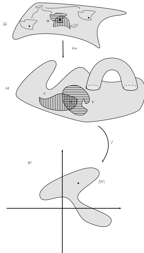
Figure 4: Constructing a chart neighbourhood in \widehat{\mathcal{M}} .
