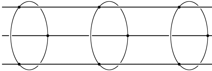
Figure 7: Part of the Cayley graph of (\mathbb{Z} \times \mathbb{Z}_3, \{(1, [0]_3), (0, [1]_3)\}) .
