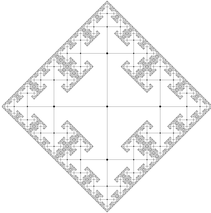
Figure 5: The Cayley graph of (\langle a, b \rangle, \{a, b\}) .
