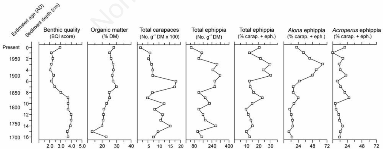
Fig. 4. Benthic quality index (BQI), sediment organic matter, total number of chydorid carapaces and ephippia, percentage of total chydorid ephippia, and proportions of ephippia of Alona affinis/quadrangularis and Acroperus harpae in the Oberer Landschitzsee core. Age estimations of the upper core (0–9 cm) are based on the age-depth model (Fig. 2) and estimations of the lower core (10–16 cm) are based on the extrapolation of the ages from the upper sediment section.
