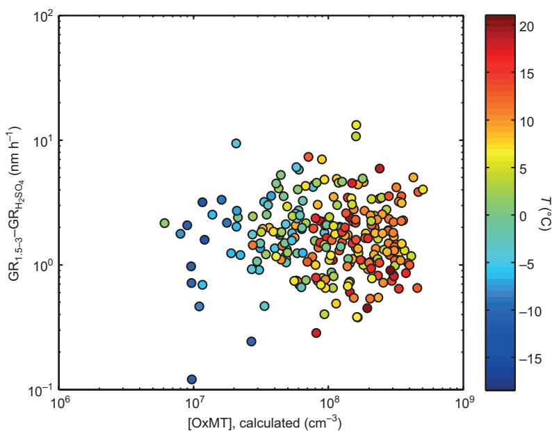
Fig. 4. Difference between the observed growth rate of 1.5–3 nm particles ( GR_{1.5-3} ) and growth rate that can be explained by sulfuric acid condensation ( GR_{H_2SO_4} ) as a function of the calculated concentration of monoterpene oxidation products during the growth time. The ambient temperature during the growth time is indicated with the color.
