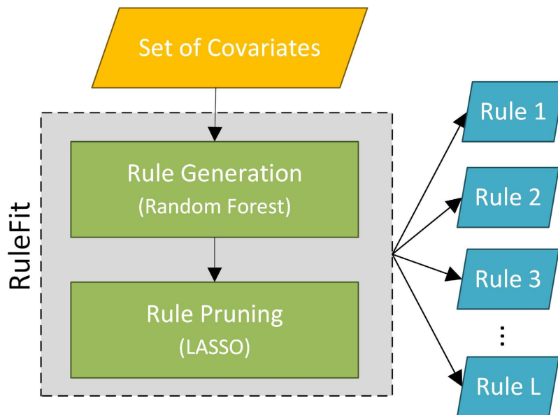
Figure 2. Flow diagram of the RuleFit algorithm.
