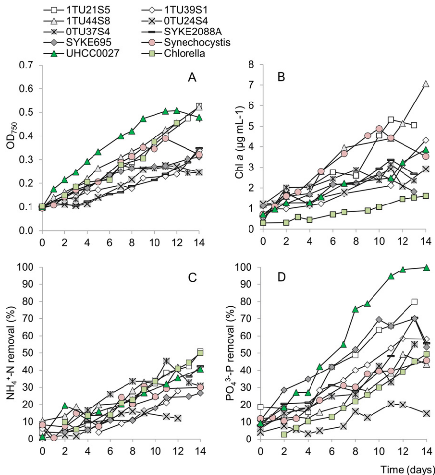
Fig. 1. Screening of cyanobacteria and algae for: biomass accumulation, as OD 750 (A) and Chl a ( \mu\text{g mL}^{-1} ) (B); and nutrient removal, as \text{NH}_4^+ -N removal (%) (C) and \text{PO}_4^{3-} -P removal (%) (D). UHCC0027 (dark green triangles), Chlorella (light green squares) and Synechocystis (light red circles) are highlighted.
