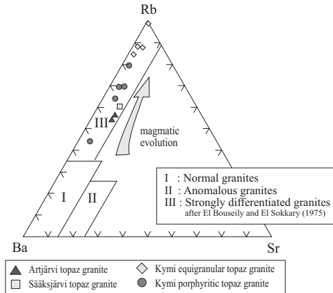
Fig. 5. Rb-Ba-Sr diagram (after El Bouseily and El Sokkary, 1975) showing the highly evolved character of the topaz granites from the Artjärvi, Sääskjärvi, and Kymi stocks.
