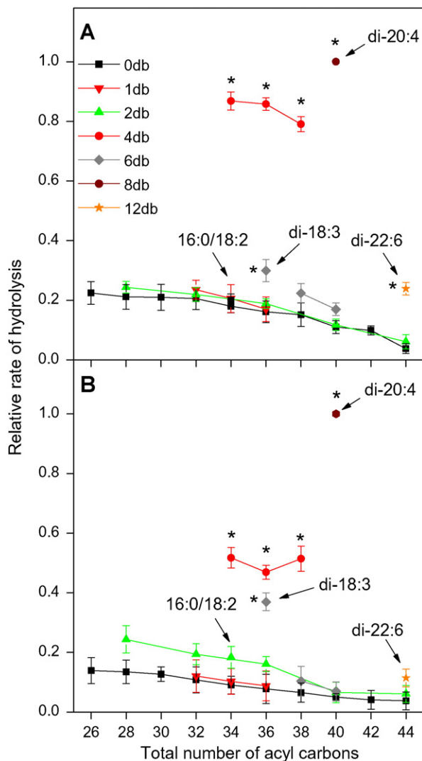
Fig. 1. Hydrolysis of PC species with varying acyl chain length and unsaturation. (A) PC-mix, 16:0/18:1-PA and 21:0-SM (250/25/25 nmol) were dispersed in 0.5 mL of assay buffer containing 1% TX-100 and incubated with 15 µg of cPLA 2 α for 30 min at 37 °C. Samples of 50 µl were drawn at intervals and the rate of hydrolysis was determined as indicated in Materials and Methods . Specific activity calculated based on the hydrolysis of di-20:4-PC was 9.8 nmol/µg protein*min. (B) Vesicles consisting of PC-mix, 16:0/18:1-PA and 21:0-SM (250/25/25 nmol) were incubated with 10 µg of cPLA 2 α in 0.5 mL assay buffer for 30 min at 37 °C and the hydrolysis was determined as above. The specific activity calculated based on the hydrolysis of di-20:4 PC was 18 nmol hydrolyzed per µg cPLA 2 /min. The sets with only a single member are indicated by an arrow. Data are mean ± S.D. of four independent experiments. db = total number of acyl chain double bonds. Statistically significant difference was found between the species marked with an asterisk and the saturated species (0 db) with the same number of total acyl chain carbons.
