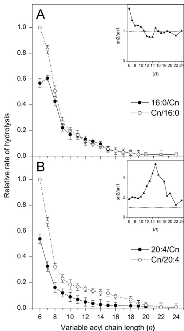
Fig. 3. Effect of the length of sn1 or sn2 chain of PC on hydrolysis in vesicle bilayers. (A) Vesicles consisting of 16:0/ C_n -PCs, D_9 - C_n /16:0-PCs, 16:0/18:1-PA and 21:0-SM (125/125/25/25 nmol) were incubated with 18 \mu g of cPLA _2\alpha in 0.5 mL of the assay buffer for 30 min at 37 °C. Specific activity calculated for the most rapidly hydrolyzed PC species was 11 nmol per \mu g cPLA _2 /min. Statistically significant differences were found only for n = 6 and 7. Inset shows an isomer preference plot obtained as indicated in the legend of Fig. 2. (B) 20:4/ C_n -PCs, C_n /20:4-PCs, 16:0/18:1-PA and 21:0-SM (125/125/25/25 nmol) incubated with 11 \mu g of cPLA _2\alpha in 0.5 mL of assay buffer for 30 min at 37 °C. The specific activity calculated for the most rapidly hydrolyzed PC species was 21.5 nmol hydrolyzed per \mu g of cPLA _2 /min. See legend of Fig. 1 for the other details. Data are mean \pm S.D. of four independent experiments. Statistically significant differences were found for n = 6 –9 and 12 and 13.
