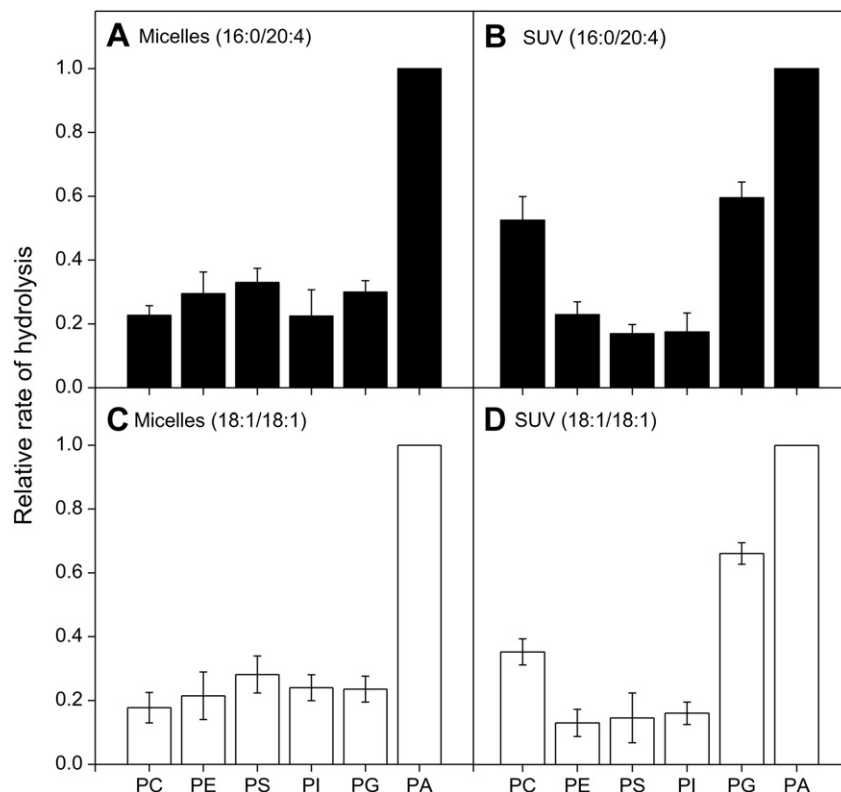
Fig. 4. Effect of the head group on GPL hydrolysis in micelles or SUV bilayers. Hydrolysis of 16:0/20:4-PE, -PS, -PI, -PG and -PA in micelles (A) or bilayers (B). Hydrolysis of 18:1/18:1-PE, -PS, -PI, -PG and -PA in micelles (C) or bilayers (D). Equimolar amounts of each GPL (250 nmol of total GPL) together with 21:0-SM (25 nmol) was incubated with 21 (A), 12 (B), 30 (C) or 18 \mu g (D) of cPLA 2 \alpha and the hydrolysis was monitored as specified in the legend of Fig. 1. The calculated specific activity was 8.0 nmol (A), 15.5 nmol (B), 4.7 nmol (C) or 8.5 nmol (D) of PA hydrolyzed per \mu g cPLA 2 /min, respectively. The differences between PA and the other GPLs are statistically significant (all panels) as it that between PC and PG vs. PE, PS and PI (panels B and D only).
