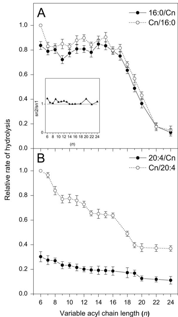
Fig. 2. Effect of the length of the sn 1 or sn 2 chain of PC on hydrolysis in Triton X-100 micelles. (A) 16:0/C n -PCs, D 9 -C n /16:0-PCs, 16:0/20:4-PC, 16:0/18:1-PA and 21:0-SM (112.5/112.5/25/25/25 nmol) were dispersed in 0.5 mL of assay buffer containing 1% TX-100 and then incubated with 24 µg of cPLA 2 α for 30 min at 37 °C. Specific activity calculated for the most rapidly hydrolysed PC species was 7.2 nmol per µg of cPLA 2 /min. Statistically significant differences were found only for n = 6 and 9. Inset shows the isomer preference vs. chain length plot obtained by pair-wise division of the rate of 16:0/C n -PC hydrolysis by that of its D 9 -C n /16:0-PC isomer. Dotted line at y = 1.0 indicates the absence of isomer preference. Note: no hydrolysis of the saturated PCs was observed in the absence of 16:0/20:4-PC or free AA (data not shown). (B) 20:4/C n -PCs, C n /20:4-PCs, 16:0/18:1-PA and 21:0-SM (125/125/25/25 nmol) were dispersed in 0.5 mL of assay buffer containing 1% TX-100 and then incubated with 15 µg of cPLA 2 α for 30 min at 37 °C. Specific activity calculated for the most rapidly hydrolysed PC species was 14.5 nmol hydrolyzed per µg cPLA 2 /min. Data are mean ± S.D. of four independent experiments. Statistically significant differences were found for all the isomer pairs. See the legend of Fig. 1 for the other details.
