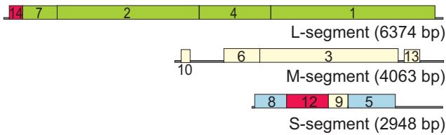
Fig. 2. Genome organization of Pseudomonas phage phi6. The gene and protein numbers are the same. Colourings indicate genes encoding constituents of the polymerase complex (green), nucleocapsid (blue), envelope-associated proteins (cream) and non-structural proteins (red).
