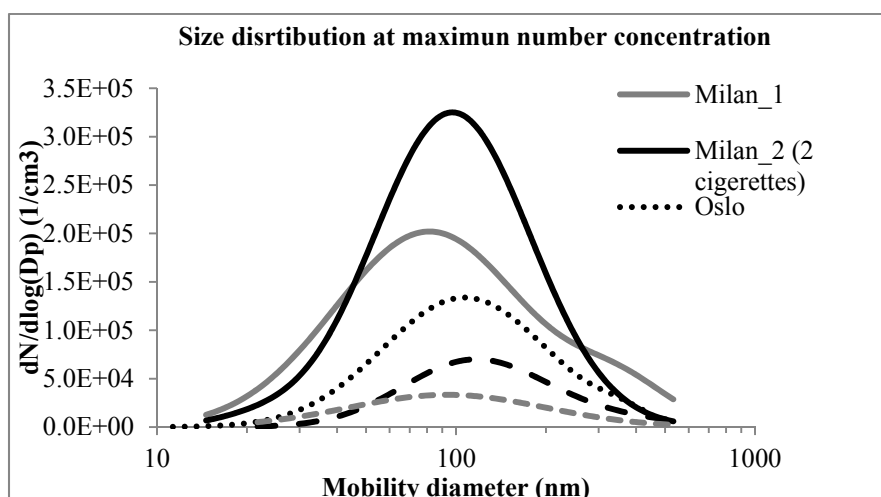
Fig. 6. Size distributions at the time of maximum number concentrations (end of emissions) during smoking in Milan (two experiments), Oslo and Prague (two experiments).
