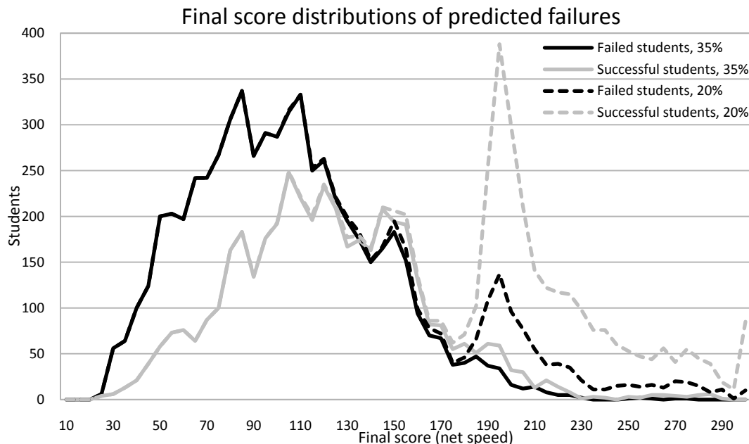
Figure 8: Regression distributions for the baseline classifier at both 35% and 20% neighbour failure
