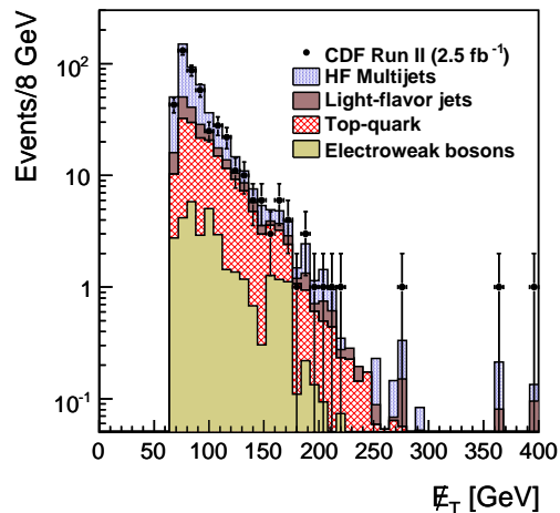
FIG. 1: Distribution of \cancel{E}_T in the pre-optimization region in which leading E_T and second-leading E_T jets are not aligned with the \vec{\cancel{E}}_T , and isolated leptons are vetoed. SM prediction (stacked histograms) and observed distribution (dots) are shown, where HF multijets and light-flavor jets are predicted from data as an integrated estimation.
