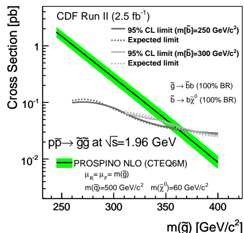
FIG. 2: Observed (solid lines) and expected (dashed lines) 95% C.L. upper limit on the gluino cross section (solid line with band) as a function of the gluino mass. The shaded band denotes the uncertainty on the NLO \tilde{g}\tilde{g} production due to the truncated higher-order terms and the parton distribution functions.
