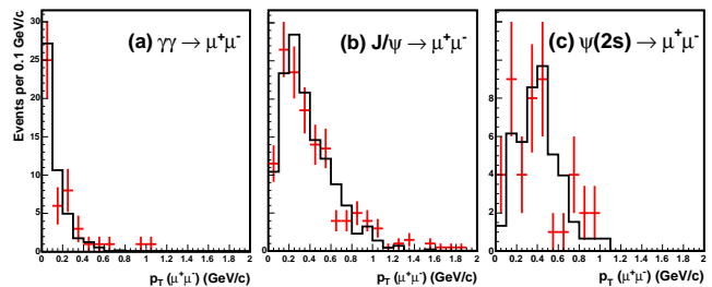
FIG. 3: p_T distribution of \mu^+\mu^- (points with statistical error bars) for (a) QED, M_{\mu\mu} \in [3.2, 3.6] \cup [3.8, 4.0] \text{GeV}/c^2 , (b) J/\psi , and (c) \psi(2S) . The MC predictions (with no background) are shown by the histograms, normalized to the data.
