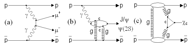
FIG. 1: Feynman diagrams for (a) \gamma\gamma \rightarrow \mu^+\mu^- , (b) \gamma\mathbb{P} \rightarrow J/\psi(\psi(2S)) , and (c) \mathbb{P}\mathbb{P} \rightarrow \chi_c , with the 2-gluon exchange forming a pomeron.
