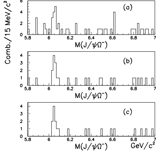
FIG. 9: The invariant mass distributions of J/\psi \Omega^- combinations for candidates with three alternative requirements for the transverse momentum of the K^- . (a) p_T(K^-) > 0.8 GeV/c. (b) p_T(K^-) > 1.2 GeV/c. (c) p_T(K^-) > 1.4 GeV/c. All other selection requirements are as in Fig. 5(c).
