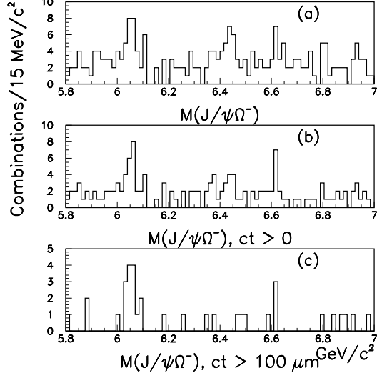
FIG. 5: (a) The mass distribution of all J/\psi\Omega^- combinations. (b) The J/\psi\Omega^- mass distribution for candidates with ct > 0 . This requirement removes half of the combinations due to prompt production. (c) The J/\psi\Omega^- mass distribution for candidates with ct > 100 \mu\text{m} . This requirement removes nearly all combinations directly produced in the p\bar{p} collision.
