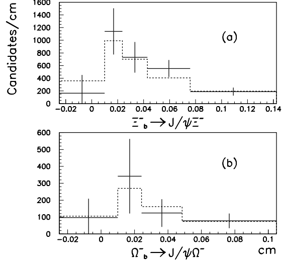
FIG. 13: The solid histograms represent the number of (a) \Xi_b^- \rightarrow J/\psi \Xi^- and (b) \Omega_b^- \rightarrow J/\psi \Omega^- candidates found in each ct bin. The dashed histogram is the fit value. Yields and fit values are normalized to candidates per cm, and the bin edges are indicated. The highest and lowest bins are not bounded, but are truncated here for display purposes.
