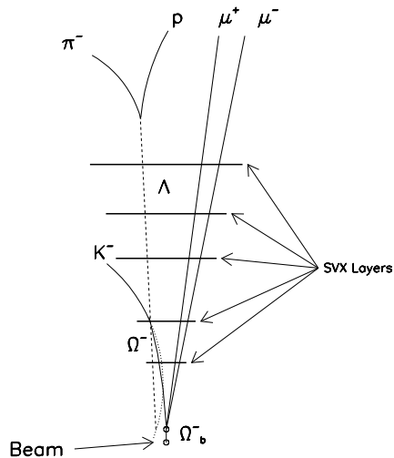
FIG. 2: An illustration (not to scale) of the \Omega_b^- \rightarrow J/\psi \Omega^- , J/\psi \rightarrow \mu^+ \mu^- , \Omega^- \rightarrow \Lambda K^- , and \Lambda \rightarrow p \pi^- final state as seen in the view transverse to the beam direction. Five charged tracks are used to identify three decay vertices. The final fit of these track trajectories constrains the decay hadrons ( J/\psi , \Omega^- , and \Lambda ) to their nominal masses and the helix of the \Omega^- to originate from the J/\psi decay vertex. The trajectory of the K^- is projected back, indicated by a dotted curve, to illustrate how an alternative, incorrect intersection with the \Lambda trajectory could exist. A comparison of the fit quality of the two \Lambda K^- intersections is used to choose a preferred solution.
