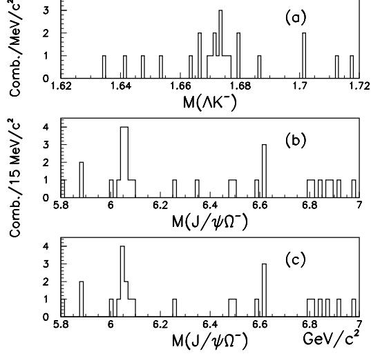
FIG. 7: (a) The invariant mass distribution of \Lambda K^- combinations for candidates with J/\psi \Lambda K^- masses in the range 6.0 - 6.1 \text{GeV}/c^2 . (b) The invariant mass distribution of J/\psi \Lambda K^- combinations for candidates with \Lambda K^- masses within 6 \text{MeV}/c^2 of the \Omega^- mass. (c) The invariant mass distributions of J/\psi \Lambda K^- combinations for candidates with \Lambda K^- masses within 4 \text{MeV}/c^2 of the \Omega^- mass. All other selection requirements are as in Fig. 5(c).
