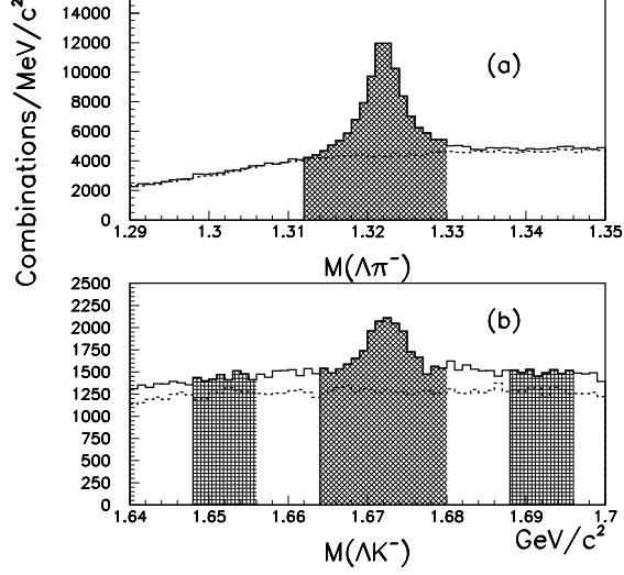
FIG. 3: The invariant mass distributions of (a) \Lambda \pi^- combinations and (b) \Lambda K^- combinations in events containing J/\psi candidates. Shaded areas indicate the mass ranges used for \Xi^- and \Omega^- candidates. The dashed histograms in each distribution correspond to \Lambda \pi^+ (a) and \Lambda K^+ (b) combinations. Additional shading in (b) correspond to sideband regions discussed in Section IV.
