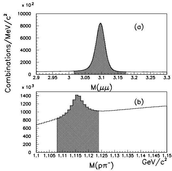
FIG. 1: (a) The \mu^+\mu^- mass distribution obtained in an integrated luminosity of 4.2 \text{ fb}^{-1} . The mass range used for the J/\psi sample is indicated by the shaded area. (b) The p\pi^- mass distribution obtained in events containing J/\psi candidates. The mass range used for the \Lambda sample is indicated by the shaded area.
