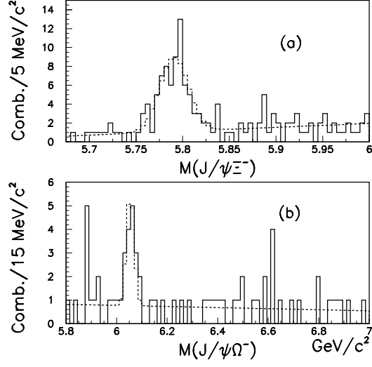
FIG. 11: The invariant mass distributions of (a) J/\psi \Xi^- and (b) J/\psi \Omega^- combinations for candidates with ct > 100 \mu\text{m} . The projections of the unbinned mass fit are indicated by the dashed histograms.
