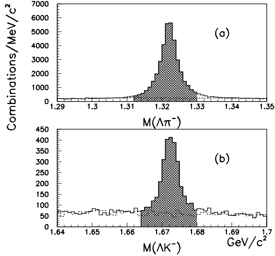
FIG. 4: The invariant mass distributions of (a) \Lambda \pi^- combinations and (b) \Lambda K^- combinations in events containing J/\psi candidates. These combinations require silicon information to be used on the hyperon track and the impact distance with respect to the primary vertex must not exceed three times its measurement resolution. Shaded areas indicate the mass ranges used for \Xi^- and \Omega^- candidates. The dashed histograms in each distribution correspond to \Lambda \pi^+ and \Lambda K^+ combinations.
