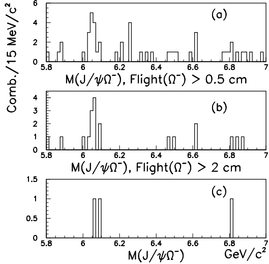
FIG. 8: (a,b) The invariant mass distribution of J/\psi \Omega^- combinations for candidates where the transverse flight requirement of the \Omega^- is greater than 0.5 cm and 2.0 cm. (c) The invariant mass distribution of J/\psi \Omega^- combinations for candidates with at least one SVXII measurement on the \Omega^- track. All other selection requirements are as in Fig. 5(c).
