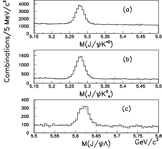
FIG. 10: The invariant mass distributions of (a) J/\psi K^*(892)^0 , (b) J/\psi K_s^0 , and (c) J/\psi \Lambda combinations for candidates with ct > 100 \mu\text{m} . The projections of the unbinned mass fits are indicated by the dashed histograms.
