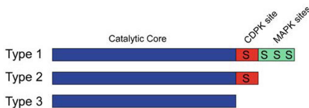
Figure 3. Cartoon representing type 1, 2, and 3 ACS proteins
