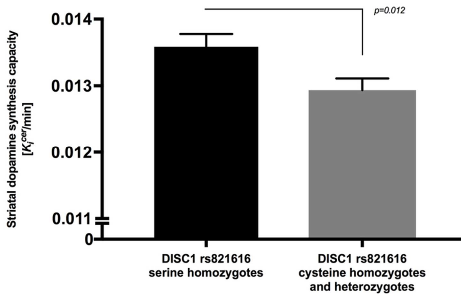
Figure 1: Mean (SEM) striatal dopamine synthesis capacity (Kicer value, min -1 ) in DISC1 rs821616 cysteine homozygotes and heterozygotes (TT and TA, N=56) and DISC1 rs821616 serine homozygotes (AA, N=46). Dopamine synthesis capacity was significantly increased in serine homozygotes compared with cysteine homozygotes and heterozygotes ( F(1,96)=6.555 , p=0.012 ).
