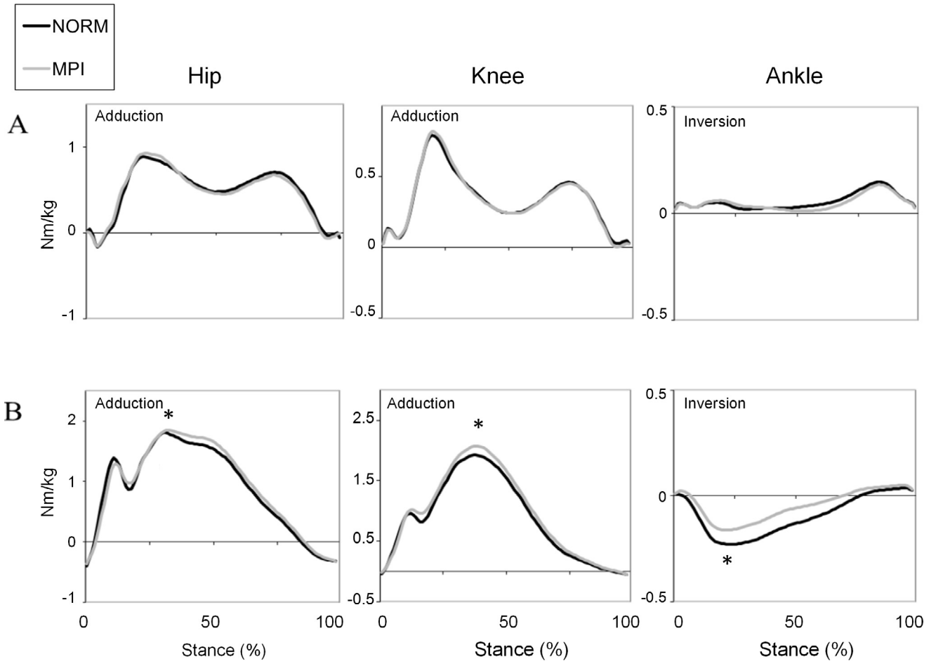
Fig. 3. External moments in the frontal plane for the hip, knee and ankle joints during walking (A) and running (B).
