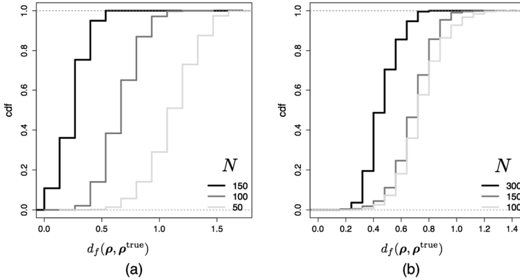
FIG. 2. Results of the simulated data. Posterior CDFs of d_f(\rho, \rho^{\text{true}}) as a function of N , for \theta = 0.1 , \alpha = 3.5 , \lambda_M = 25 , n = 15 (a), and for \theta = 0.1 , \alpha = 4.5 , \lambda_M = 50 , n = 25 (b).
