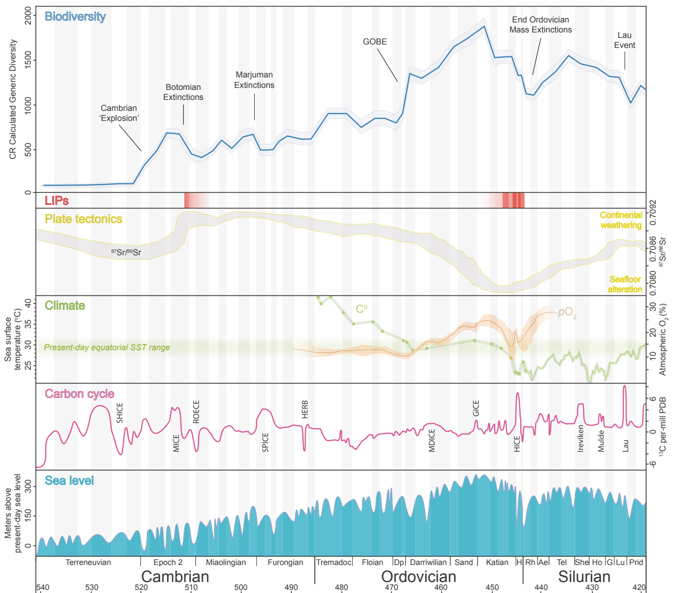
Fig. 2. Generic biodiversity history for the Early Paleozoic based on an average estimate after 50 model runs using the CR method. The temporal resolution of the dataset is shown by the alternating gray/white bars corresponding to the 53 time slices partitioned on the basis of biostratigraphically defined boundaries and matched with lithostratigraphical information extracted from the Paleodb. Confidence intervals envelope the blue richness line. Major biotic events are annotated. In addition, Early Paleozoic biodiversity accumulation is set in the context of potential abiotic determinants. The sea level and strontium trends overall mirror the richness curve, reflecting that plate tectonics is a first-order determinant on speciation. The main radiation during the GOBE correlates strongly to cooling climate and a rise in oxygen levels. However, these determinants do not seem to accelerate biodiversity accumulation during the Silurian. Last, note the apparent association between Large Igneous Provinces (LIPs), abrupt, positive ^{13}\text{C} values, and extinctions phases, suggesting a volcanic component in these intervals. Strontium isotope data are based on the LOWESS fitted line (77); LIPs are based on refs. 78–82, with darker red bands corresponding to large volcanic eruptions (69, 83–85); climate proxies are based on refs. 33, 35, and 63; the ^{13}\text{C} record is compiled from ref. 11, and sea level is based on refs. 30, 32, 72, and 86.
