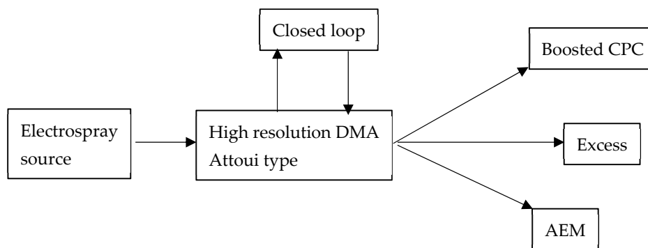
Figure 1. Experimental set up used in this study.
