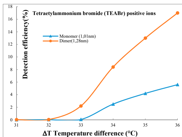
Figure 7. Detection efficiency of the CPC for TEABr and TBABr ions for different \Delta T s.
