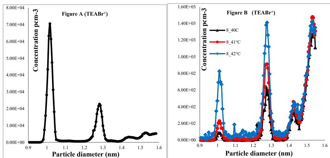
Figure 5. Mobility measurements of the tetraethylammonium bromide (TEABr) with a DMA. Aerosol electrometer was in use in the results given in the Figure A (left panel). Variable \Theta T CPC was in use for the results given in the Figure B (right panel).
