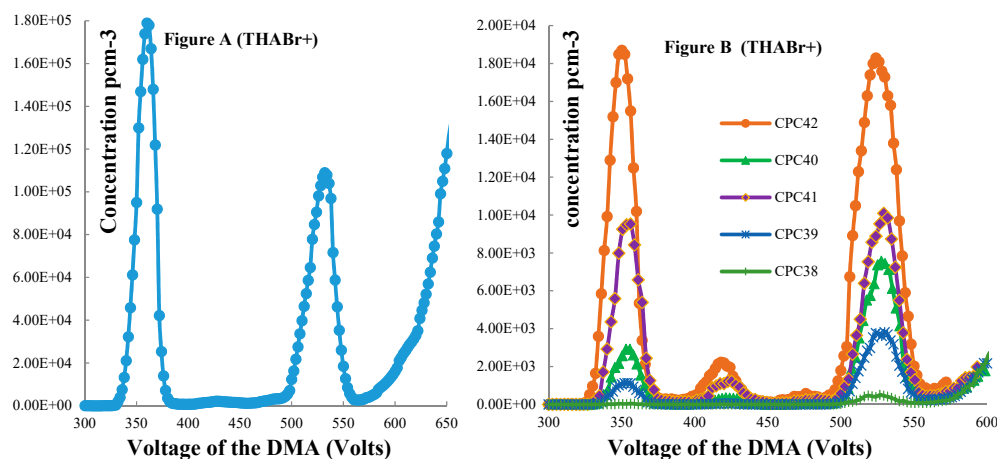
Figure 3. Mobility diameter distribution measurements of the tetraheptylammonium bromide as a function of the voltage of the DMA. Aerosol electrometer (AEM) was in use in the results given in the Figure A (left panel). Variable saturator temperatures CPC was in use for the results given in the Figure B (right).
