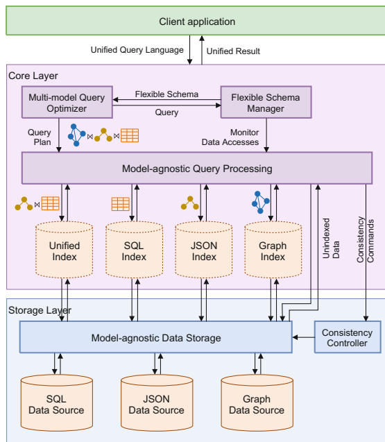
Fig. 1. Architecture of the UDBMS.
