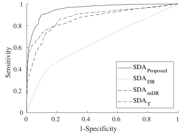
Figure 3. SDA performance against human consensus ( n=39 , neonates with seizure): sensitivity as a function of 1-specificity, averaged over seizure patients.
