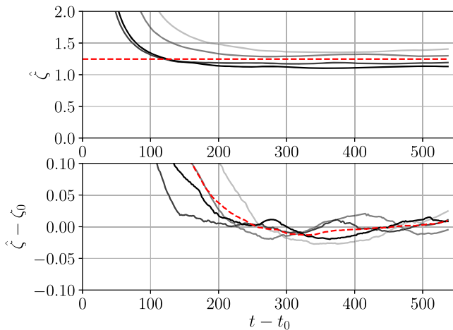
FIG. 2. Top: String length density parameter \hat{\zeta} [see Eq. (5)] plotted against offset time t - t_0 , for all 4k runs with initial correlation length \ell_\phi = 5 . The dashed line shows the mean of \zeta_0 = 1/4\beta^2 . Bottom: Residuals ( \hat{\zeta} - \zeta_0 ) plotted against offset time t - t_0 , for the same simulations. Individual runs are shown in solid lines and the residuals between the mean \zeta_0 and \hat{\zeta} in dashed lines.
