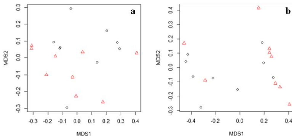
Fig. 1 NMDS ordination of bacterial communities at the a) phylum level (stress = 0.06), b) order level within the phylum Actinobacteria (stress = 0.04) in shiro soil (open circles), non-shiro soil (open triangles) samples
