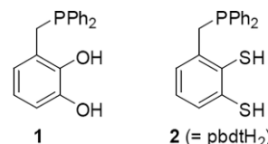
Scheme 1. Ditopic ligands 1 and 2 (pbdtH 2 = phosphane-benzenedithiol).
