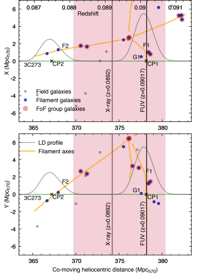
Fig. 7. Filament analysis for 3C 273 sight-line near z = 0.09 . The figure shows the distribution of SDSS galaxies (points) in two orthogonal projections ( upper and lower panels ), each of which are 20 Mpc thick. Blue points represent galaxies in filaments and red points indicate additional galaxies in friends-of-friends groups. The detected filament axes F1 and F2, and the associated luminosity density profiles are denoted by yellow lines and grey curves, respectively. The crossing points of the filaments F1 and F2 and the sight-line to 3C 273 are denoted with labels “CP1” and “CP2”, respectively. The redshift of the O VI absorption is marked with the black vertical line, whereas the pink vertical line and area correspond to the X-ray measured O VII line centroid and its 1\sigma measurement uncertainty, obtained in the Gaussian model fit to the O VII Ly \alpha feature (see Table 4)
