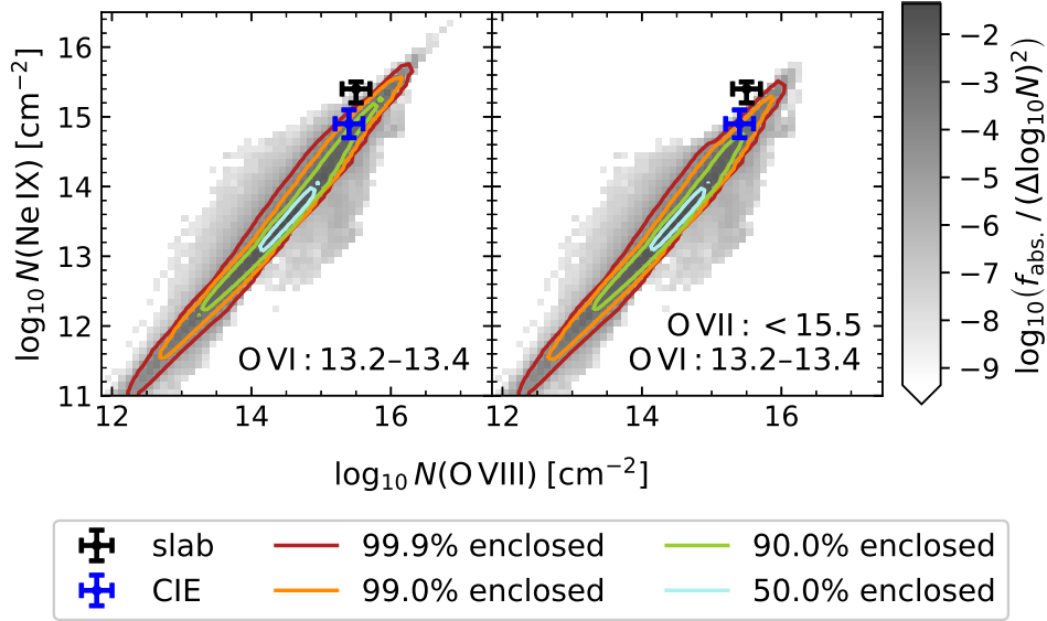
Fig. 9. Distribution of O VIII and Ne IX column densities in counterparts to O VI absorbers (grayscale and contours) according to the EAGLE simulation, compared to the measured column densities at z = 0.09 for the CIE and slab models. Left panel: counterparts to O VI absorbers with column densities of 10^{13.2}-10^{13.4} \text{ cm}^{-2} , which is roughly the \pm 1\sigma range for the FUV absorber of Tilton et al. (2012). Right panel: subset of O VI counterparts with an O VII column density in agreement with the upper limit measured with the slab model. The contours enclose different fractions of the counterparts, as indicated in the legend, while the grayscale shows the fraction of all EAGLE absorbers satisfying the indicated constraints. Although most EAGLE O VI absorbers have weaker (and hence undetectable) associated Ne IX and O VIII absorption than observed at z = 0.09 (but consistent with the non-detection for the z = 0.12 O VI absorber), both the “slab” and CIE measurements are consistent with EAGLE at the \approx 1-2\sigma level. The O VII upper limit does not affect the distribution much.
