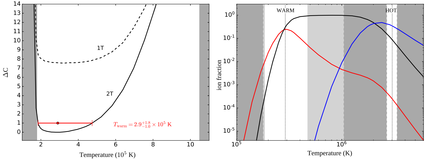
Fig. 8. Thermal properties of the absorbing gas at z = 0.09017 assuming CIE. Left: temperature dependence of the two-phase absorption model fit statistics to the X-ray data (black solid curve) when N_{\text{OVI}} is fixed to the FUV measured value. The shaded areas mark the forbidden regions based on the FUV measurements (the lower limit is yielded by the limits on N_{\text{CIII}} and N_{\text{OVI}} , whereas the upper limit is set by the O VI line broadening). The 1T curve shows the X-ray model fit statistics without the hot absorption component included, and is plotted for reference. Right: O VI (red), O VII (black) and O VIII (blue) ion fractions over the T -ranges of the warm and hot CIE components. The dotted lines mark the best-fit temperatures for both phases, while the white regions mark the 1\sigma uncertainty limits as yielded by X-ray data. The light gray shaded regions show the improvement which X-ray data provides to the T_{\text{warm}} determination as compared to the limits obtained with FUV data.
