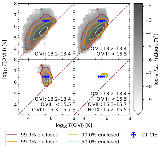
Fig. 10. Distribution of O VI- and O VIII-weighted temperatures in counterparts to O VI absorbers (grayscale and contours) according to the EAGLE simulation, compared to the best-fit temperatures at z = 0.09 for the 2-temperature CIE model (warm and hot phase, respectively). From left to right, top to bottom, we show how constraints on the column densities of different ions from the “slab” model affect the temperatures of O VI and O VIII absorbers in EAGLE. Column density ranges are shown in units of \log_{10} \text{ cm}^{-2} for the different ions. The O VI constraints are from Tilton et al. (2012). The contours enclose different fractions of the absorbers in each column density selection, as indicated in the legend, while the grayscale shows the fraction of all EAGLE absorbers satisfying the indicated constraints. The brown dashed line indicates where the temperatures are equal. Most absorbers are multiphase and the 2T CIE model is consistent with EAGLE.
