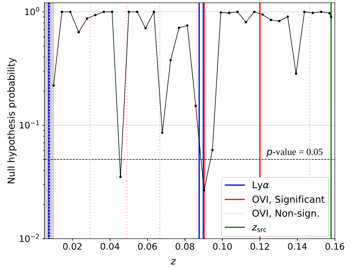
Fig. 2. Statistical probability of the Null hypothesis validity over the redshift range 0.005–0.158. The Null hypothesis is the emission model with Galactic absorption, which is compared to the WHIM hypothesis, i.e., a model including a redshifted hot ( T = 10^{6-7} K) CIE absorption component. The dashed black line marks the commonly adopted Null hypothesis rejection limit, p = 0.05 . The FUV redshifts listed in Table 1 are shown together with the non-significant O VI doublet detections (from Table 4 in Tilton et al. 2012). The shaded color marks the confusion region of the redshifted absorption component with the Galactic hot halo.
