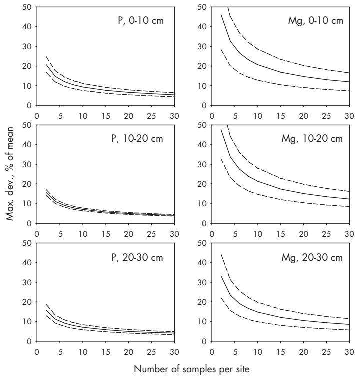
Fig. 3. Theoretical maximum deviations of total P and Mg concentration estimates (sample means) from population means in different peat layers (sampling depths) relative to the number of samples taken per site. Solid line = mean of all 11 sites, dashed lines = 95% confidence limits.
