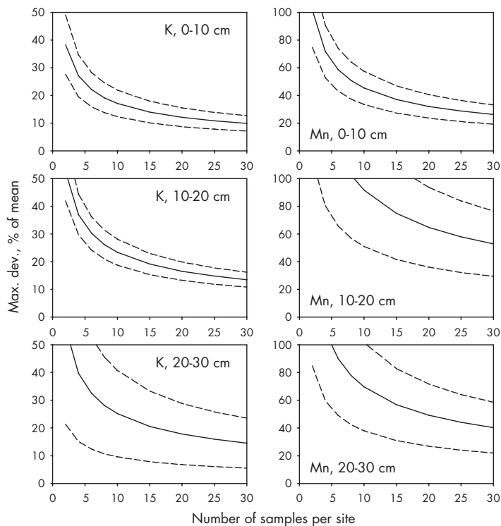
Fig. 4. Theoretical maximum deviations of total K and Mn concentration estimates (sample means) from population means in different peat layers (sampling depths) relative to the number of samples taken per site. Solid line = mean of all 11 sites, dashed lines = 95% confidence limits. Note the difference in y-axis scales between K and Mn.
