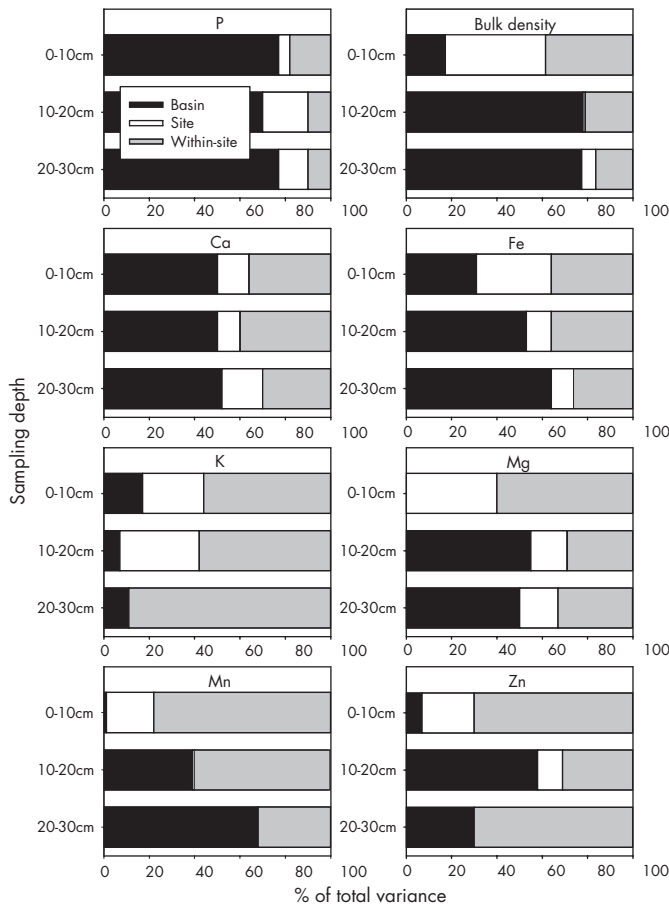
Fig. 1. Proportions of total variance, %, contributed by different hierarchical levels (peatland basin, site, and within-site variation) at different sampling depths.
