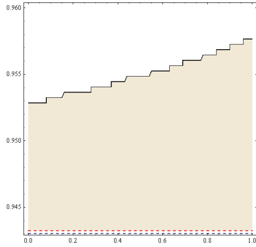
Figure 5C: Domain of attraction with X_0 = 0.95 in a boom like scenario. Credibility along horizontal axis and output expectations along vertical axis.
