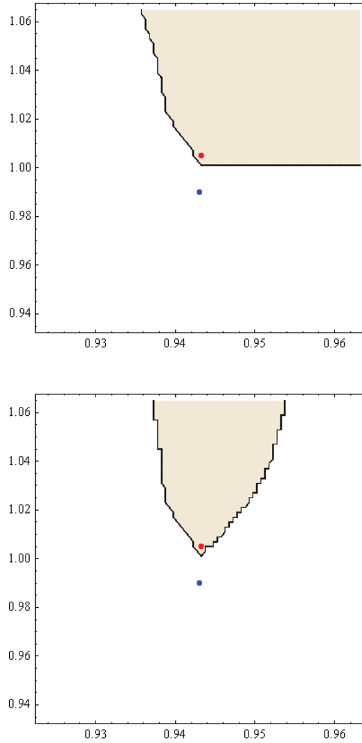
Figure 1: Domain of attraction for IT (top panel) and that for PLT without guidance (bottom panel). Horizontal axis gives y_0^e and vertical axis \pi_0^e . Shaded area indicates convergence. The circle in the shaded region denotes the intended steady state and the circle outside the shaded region denotes the unintended steady state.
