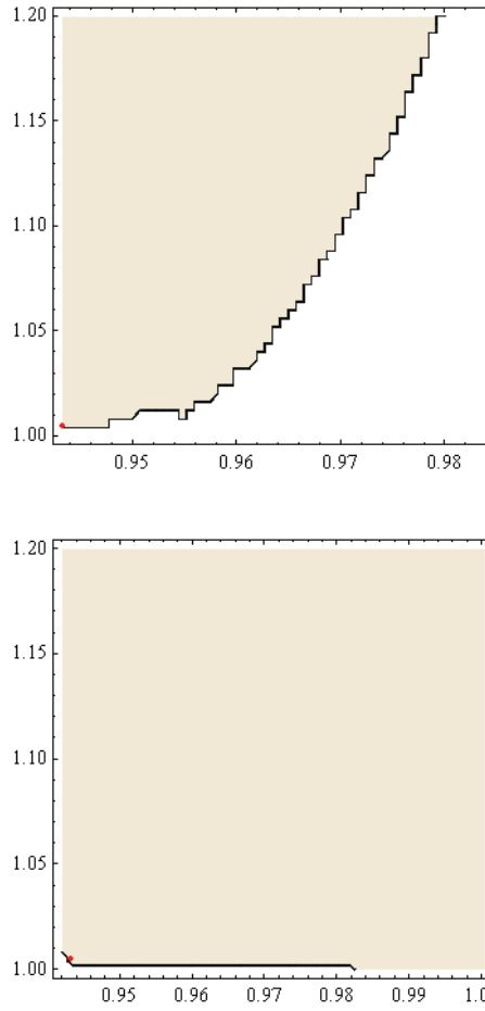
Figure 4: The top panel shows the domain of attraction for PLT with high credibility ( q_0^C = 0.9 ) and the bottom panels shows the domain for IT. Output expectations are along the along horizontal axis and inflation expectations along vertical axis. Note that output expectations above 0.98 are not stable with PLT whereas even output expectations as high as one are stable with IT.
