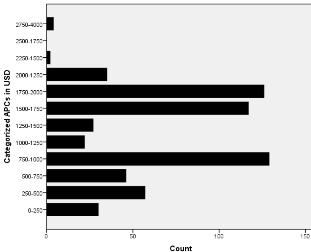
Figure 1. The distribution of APCs across journals
