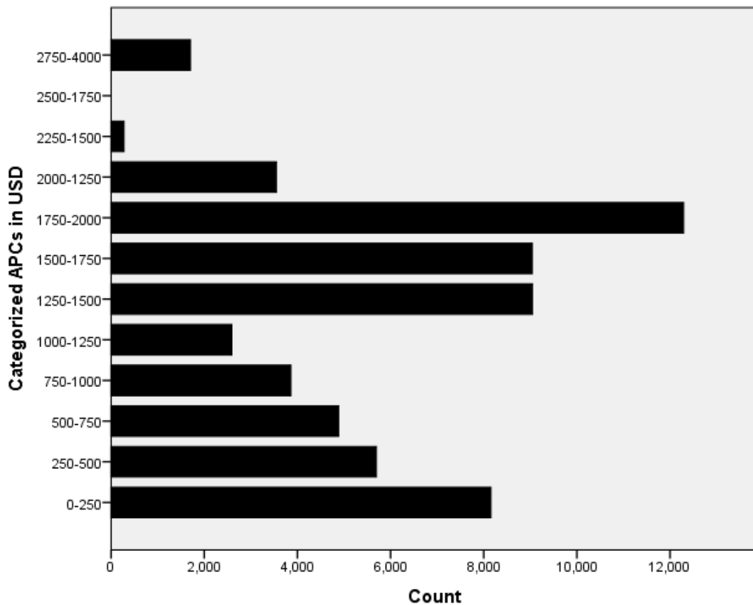
Figure 2. The distribution of APCs across articles
