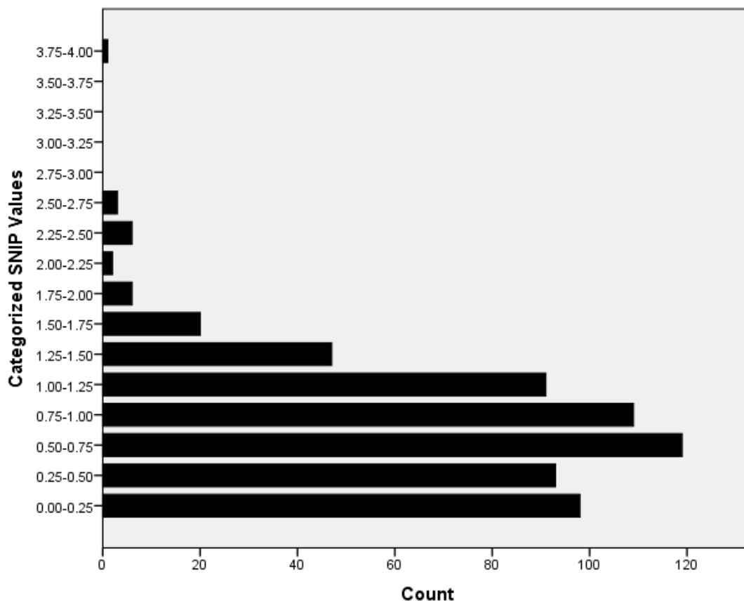
Figure 3: Distribution of SNIP levels for journals.
