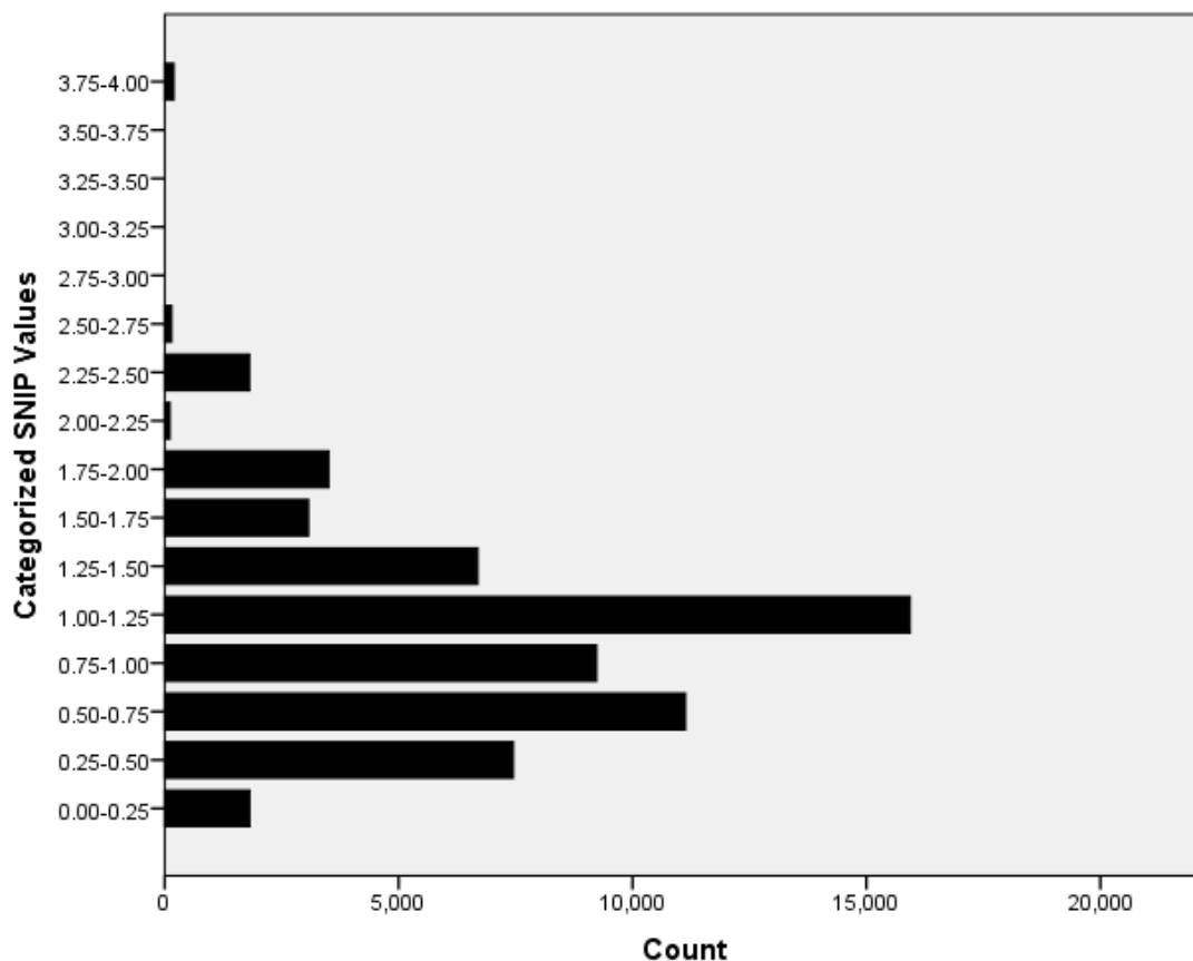
Figure 4. The distribution of SNIP values across articles
