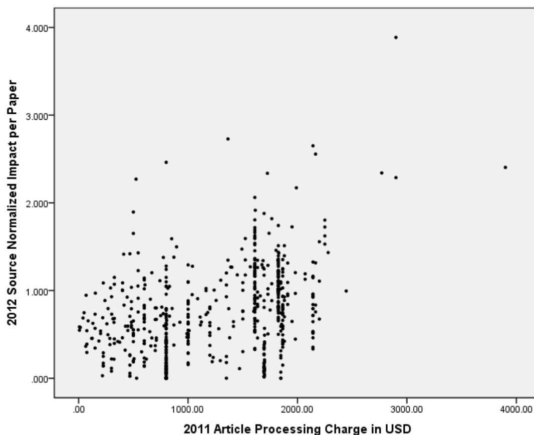
Figure 5. Scattergram of the distribution of APC and SNIP values. The three long vertical lines represent the journals of a couple of publishers with single or two-tier prices.
