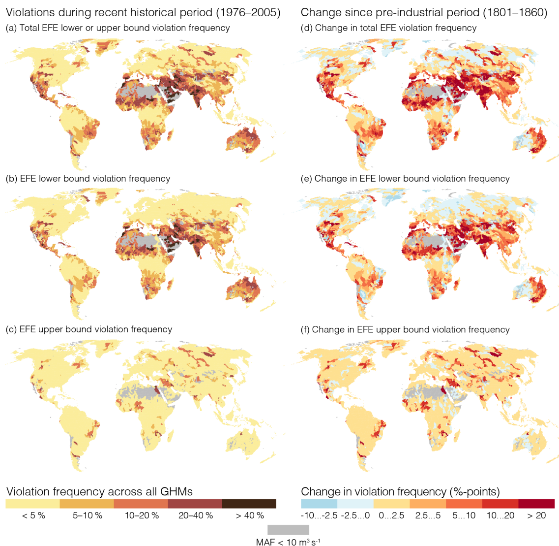
Figure 2. Frequency of environmental flow envelope (EFE) violations during the recent historical period (1976–2005); for both upper and lower bounds (a), lower bound only (b), and upper bound only (c), aligned with the change in violation frequency since the pre-industrial period (1801–1860) (d–f). All values are computed across four global hydrological models (GHMs). Sub-basins with mean annual flow (MAF) less than 10 m 3 s -1 at the sub-basin outlet are excluded. Case examples of how the recent historical discharge compares with the EFE in different flow regimes are shown in Fig. A3.
