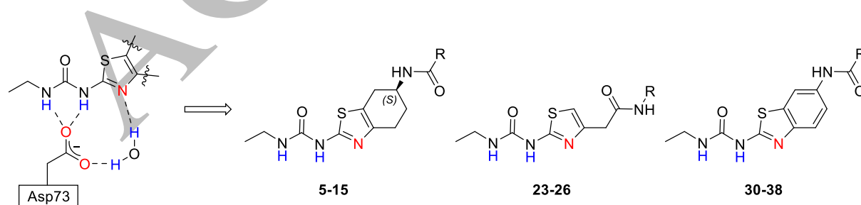
Figure 2. The hydrogen bonds of the thiazole-based ethylureas in the ATP binding site of DNA gyrase ( E. coli numbering) and designed novel thiazole-based ethylurea DNA gyrase B inhibitors.
