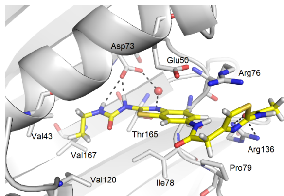
Figure 3. The docking binding mode of inhibitor 34 (in yellow ) in the ATP binding site of E. coli DNA gyrase B (in grey , PDB code: 4DUH [32]). The ligand and the neighbouring protein side-chains are shown as stick models, coloured according to the chemical atom type (blue, N; red, O; orange, S; green, Cl). Water molecule is presented as a red sphere. Hydrogen bonds are indicated by black dotted lines.
