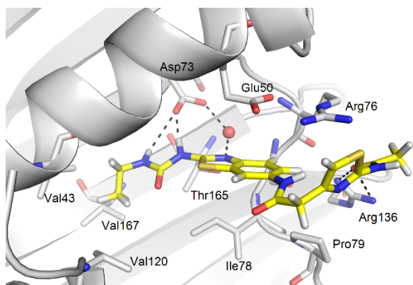
Figure 3. The docking binding mode of inhibitor 34 (in yellow) in the ATP binding site of E. coli DNA gyrase B (in grey, PDB code: 4DUH [29]). The ligand and the neighbouring protein side-chains are shown as stick models, coloured according to the chemical atom type (blue, N; red, O; orange, S; green, Cl). Water molecule is presented as a red sphere. Hydrogen bonds are indicated by black dotted lines.
