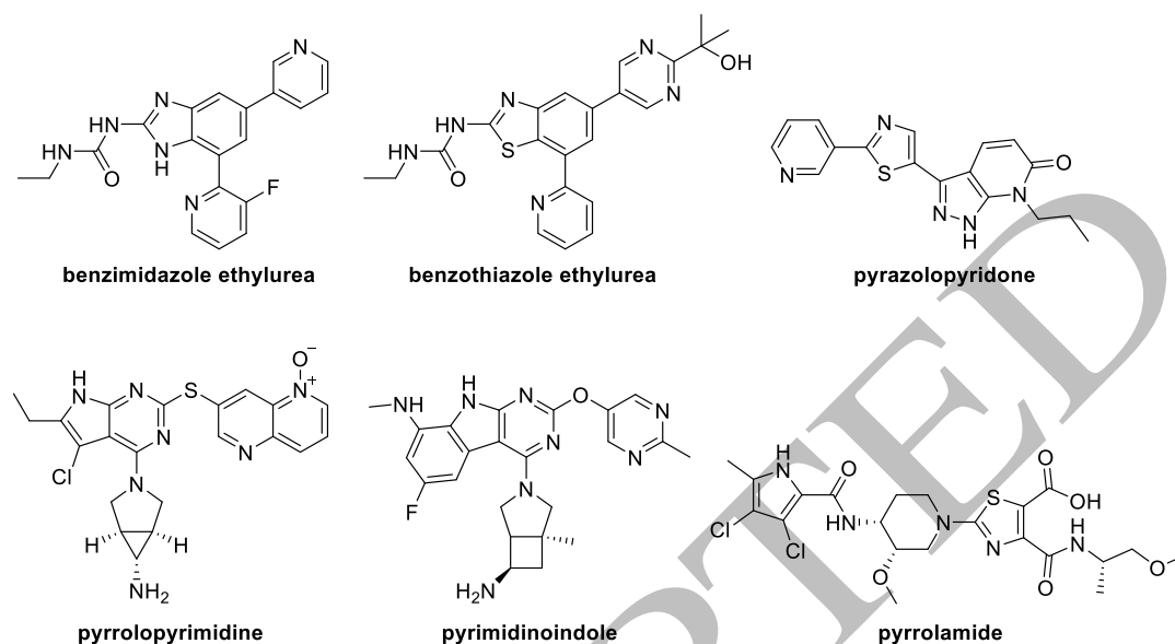
Figure 1. Representative synthetic GyrB and/or ParE inhibitors.
