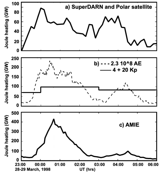
Figure 2. Discrepancies between global integrated Joule heating as estimated by (a) SuperDARN and Polar measurements, (b) AE- and Kp-based proxies, and (c) the AMIE procedure during a solar storm (adapted from Palmroth et al., 2005).
