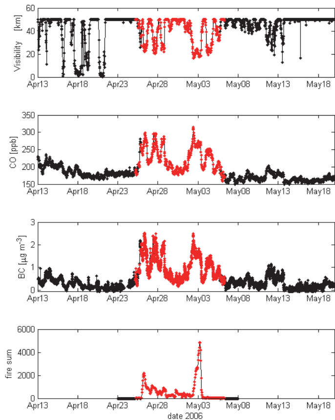
Fig. 2. Visibility, CO concentration, black carbon concentration and “fire sum” in Hyttiälä in spring 2006. Hours when the “fire sum” was positive are marked in red and indicate the spring smoke episode in Hyttiälä.
