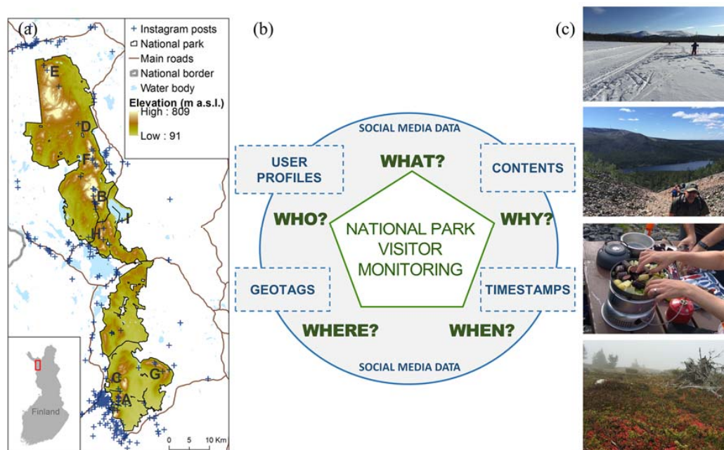
Figure 1. (a) Instagram post locations from the case study area of Pallas-Yllästunturi National Park (PY) in Finnish Lapland; (b) Framework for using social media data (geotags, timestamps, contents, user profiles) for studying the spatial patterns (where), temporal patterns (when) of visitors/social media users (who) and their activities (what), and motivations (why) (modified from [14]); and (c) examples of social media image content from the national park.
