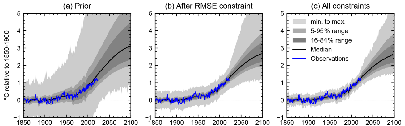
Figure 9. Progression of projections using the historical + harmonised SSP2-4.5 emissions for (a) all prior ensemble members, (b) the RMSE < 0.17^{\circ}\text{C} first constraining step, and (c) the final reweighted and constrained posterior. In each plot, progressively darker shaded regions correspond to the minimum–maximum, 5 %–95 %, and 16 %–84 % ranges. The black line is the ensemble median, and the blue line is a historical best-estimate GMST from the Indicators of Global Climate Change 2022 (Forster et al., 2023).
