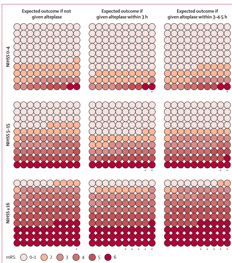
Figure 5: Expected stroke outcome at 3–6 months for different groups of patients mRS 0–1 indicates an excellent outcome: survival symptom free or residual symptoms with no loss of activity. mRS 5–6 indicates bed bound or dead at 3–6 months. Each 10 × 10 grid represents 100 hypothetical patients who have had a stroke with severity 0–4 NIHSS points, 5–15 points, or 16 or more points. mRS=modified Rankin Scale. NIHSS=National Institutes of Health Stroke Scale. *Death within 7 days and after a type 2 parenchymal haemorrhage.
