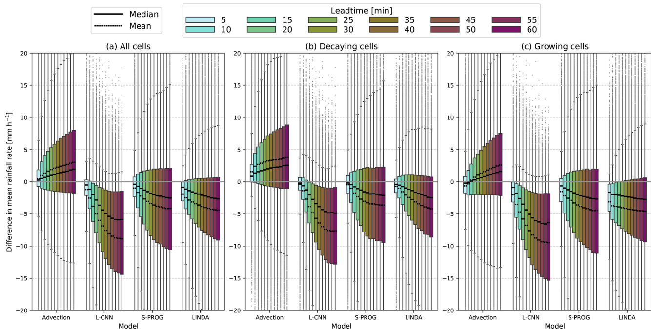
Figure 12. Box plots of differences between predicted and observed mean rain rate inside the cells by nowcast lead time for (a) all cells, (b) decaying cells, and (c) growing cells. The boxes show the 25th to 75th percentile range, while the whiskers represent the 5th to 95th percentile range. The solid line indicates the median, the dotted line is the mean, and outliers are indicated by dots. A positive difference indicates overestimation of the mean rain rate by the model, whereas a negative difference denotes underestimation.
