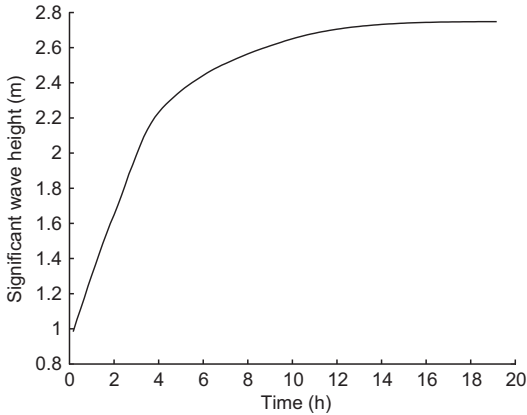
Fig. 3. Dependence of significant wave height on wind duration at the Harilaidi Bank.
