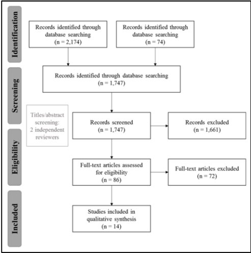
Figure 1. PRISMA diagram
