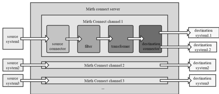
Figure 1. Messaging-process flow.
