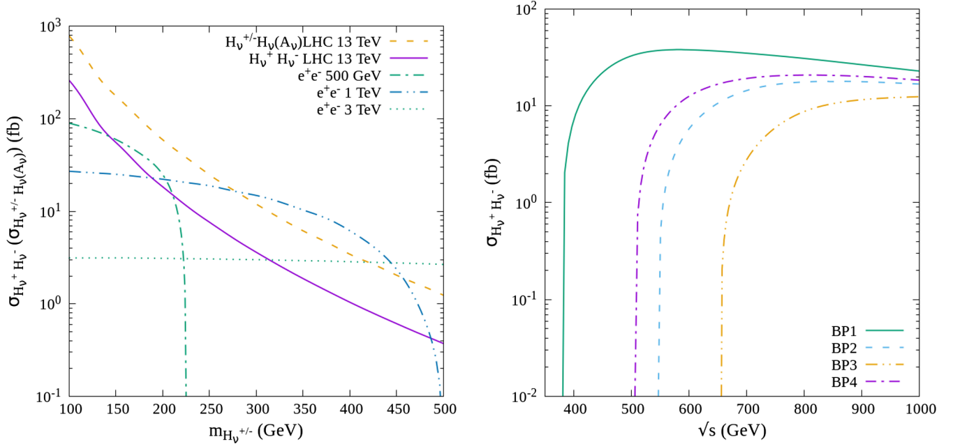
FIG. 4. Variation of the charged Higgs pair production cross section at the LHC and an e^+e^- collider at center-of-mass energies of 13 and 1 TeV, respectively. The distribution on the right shows variation of the charged Higgs pair production cross section at an e^+e^- collider with varying center-of-mass energy ( \sqrt{s} ) for our four benchmark points.
