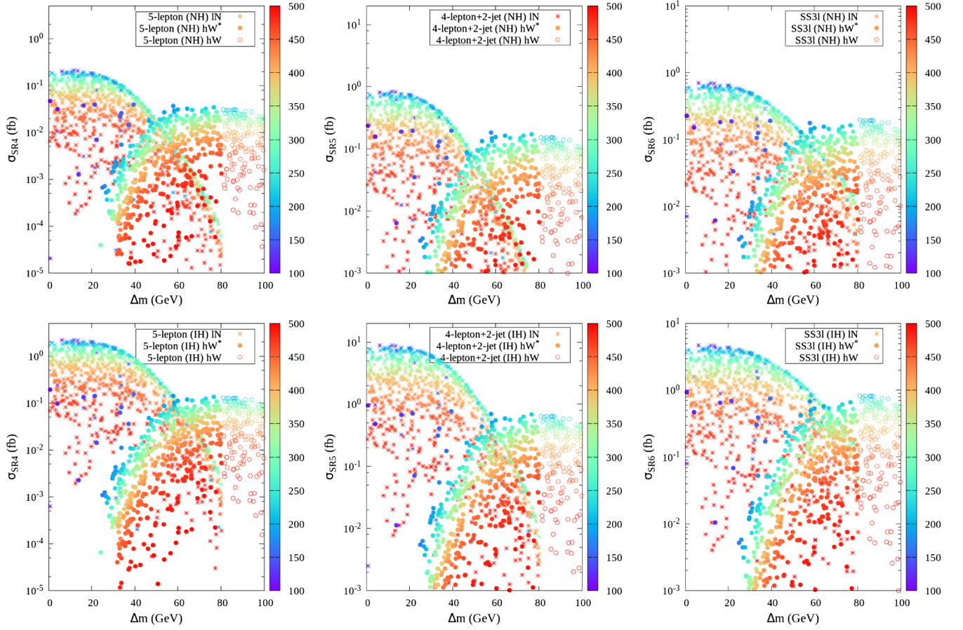
FIG. 7. Variation of cross sections corresponding to the signal regions SR4 , SR5 , and SR6 as a function of \Delta m at an e^+e^- collider with 1 TeV center-of-mass energy. The two rows represent scenarios with normal and inverted hierarchies of the light neutrino masses, respectively. The color coding represents variation of m_{H_{\nu}^{\pm}} . For all points, heavy neutrino masses are kept at 100 GeV.
