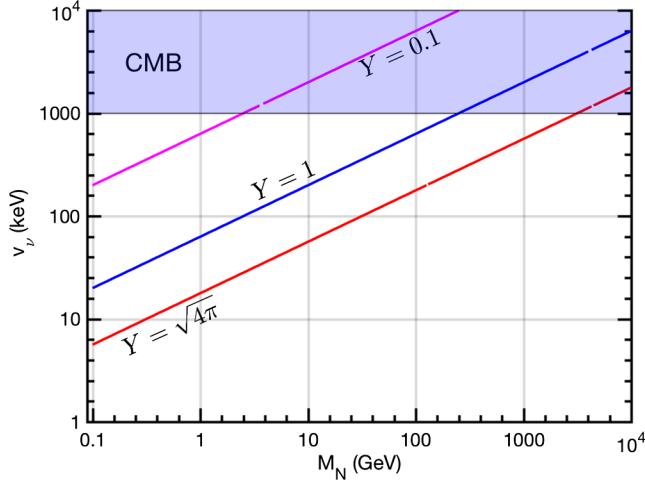
FIG. 2. Yukawa contours on the (M_{N_i}, v_\nu) plane. The lines corresponding to the neutrino Yukawa couplings Y = 0.1, 1, \sqrt{4\pi} are drawn. Below the red Y = \sqrt{4\pi} line, the theory is non-perturbative. Blue-shaded region denoted “CMB” is excluded due to restrictions of CMB temperature anisotropies induced by domain walls. The available parameter space is restricted also from BBN requirement M_{N_i} \gtrsim 0.1 GeV.
