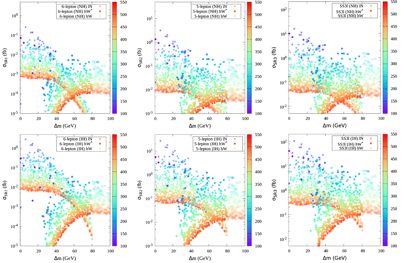
FIG. 6. Variation of cross sections corresponding to the signal regions SR1 , SR2 , and SR3 as a function of \Delta m at 13 TeV LHC. The two rows represent scenarios with normal and inverted hierarchies of the light neutrino masses, respectively. The color coding represents variation of m_{H_v^\pm} . For all points, heavy neutrino masses are kept at 100 GeV.
