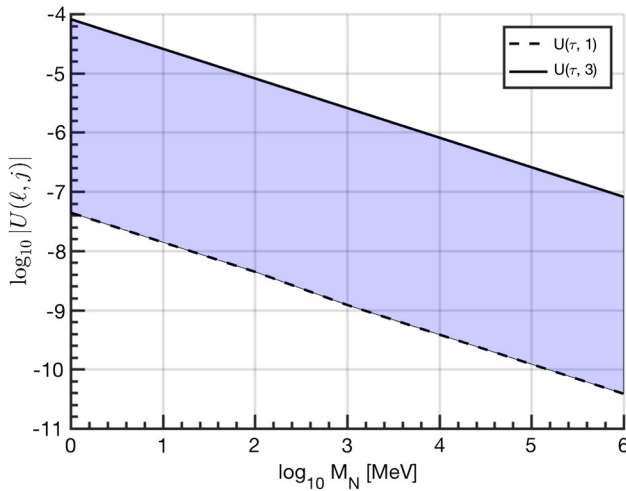
FIG. 1. Absolute values of active-sterile mixing block matrix elements as a function of heavy neutrino mass M_N . All the active-sterile elements fall in the blue band.
