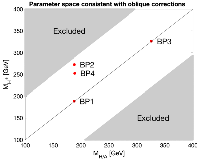
FIG. 5. In the gray region, the oblique corrections induced by the neutrinophilic Higgses are too large. A too large mass difference \Delta m \equiv m_{H_{\nu}^{\pm}} - m_{H_{\nu}, A_{\nu}} is disfavored. Red dots label the chosen benchmark points. The black line corresponds to m_{H_{\nu}^{\pm}} = m_{H_{\nu}, A_{\nu}} .
