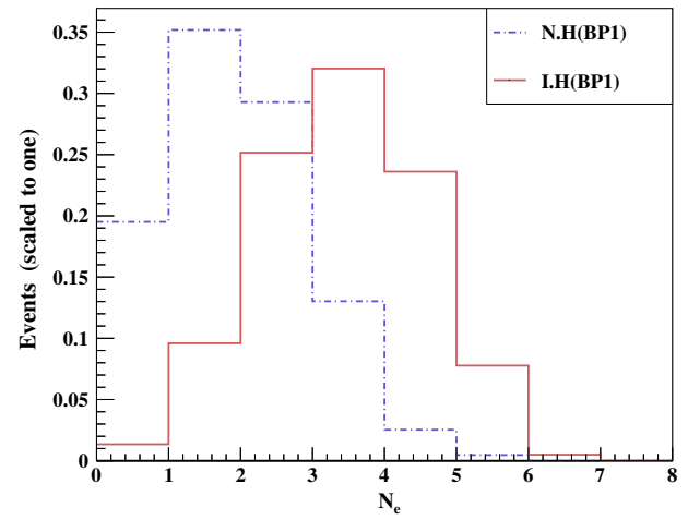
FIG. 8. Electron multiplicity distribution for BP1 in normal and inverted hierarchy scenarios indicated by blue and red lines respectively. The distributions correspond to the choice of final states as per SR2 .
