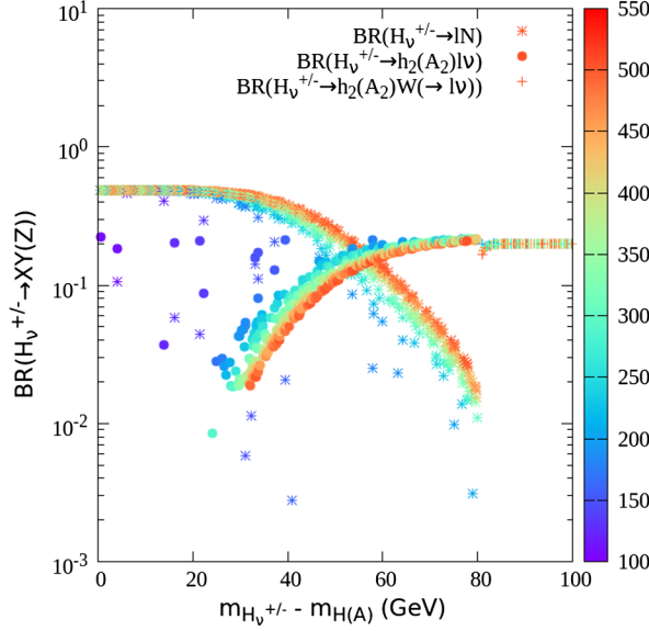
FIG. 3. Variation of \text{BR}(H_\nu^\pm \rightarrow N\ell^\pm) , \text{BR}(H_\nu^\pm \rightarrow H_\nu(A_\nu) \times W^\pm(\rightarrow \ell^\pm \nu)) , and \text{BR}(H_\nu^\pm \rightarrow H_\nu(A_\nu)\ell\nu) as a function of \Delta m . The color coded bar on the right shows the variation of m_{H_\nu^\pm} . For all the points, m_N is kept fixed at 100 GeV. Normal hierarchy is assumed for the light neutrinos. For inverted hierarchy, although the numerical values of the BRs are expected to be different, the pattern of the distribution remains the same.
