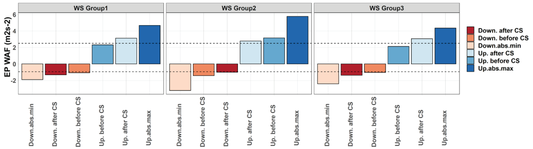
Fig. 10. Intensity of upward and downward Eliassen-Palm WAFs (averaged 30 days before the WS, the averaged absolute maxima and minima, and WAF intensity averaged 20 days after the start of the WS) during the 1981–2020 period. The dashed horizontal lines accordingly show the long-term (1981–2020) mean values of November–February maxima upward and minima downward WAFs.
