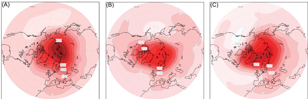
Fig. 3. Average GPH anomalies (m) at a 10 hPa pressure level (a) 30 days before the CS; (b) 20 days before the CS; and (c) 10 days before the CS in the NH (20–90°N).
