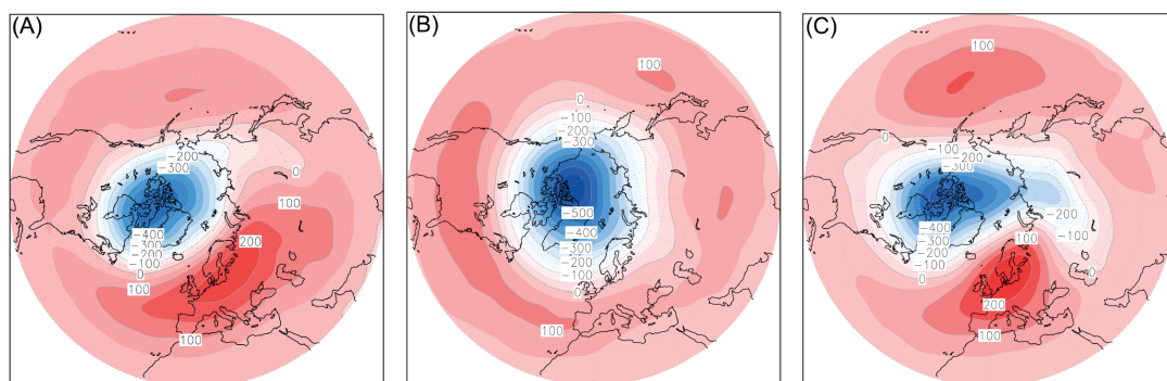
Fig. 5. Average GPH anomalies (m) during non-stratospheric CSs at 10 hPa pressure level (a) 30 days before CS; (b) 20 days before CS; and (c) 10 days before CS in the NH (20–90°N).
