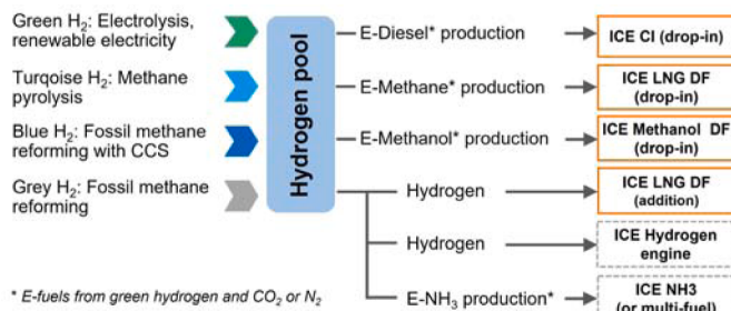
Fig. 9. Hydrogen pathways for ICE include fuels compatible with common diesel and gas engines (hydrogen-based e-fuels as drop-in). Hydrogen and ammonia ICE engines are not on market for marine applications, yet (marked with a dashed line).
