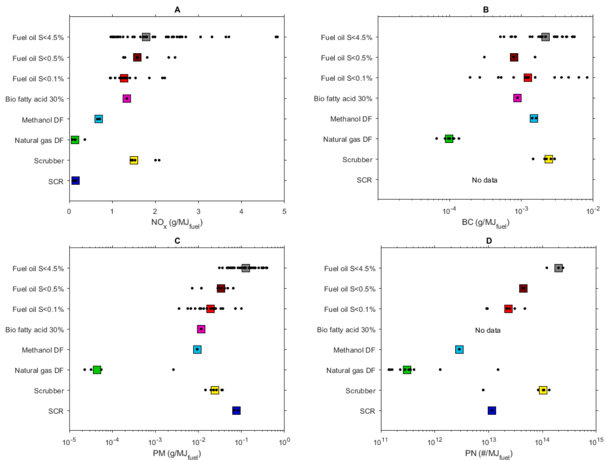
Fig. 6. Emissions from marine engines using different fuels and exhaust gas treatment technologies. MSD and SSD engines, engine loads equal or above 40% MCR: a) \text{NO}_x emissions. b) BC emissions. c) PM emissions. d) PNv emissions (non-volatile). Small markers represent individual data points and large coloured markers represent the median values. Grey: S < 4.5\% fuel. Dark red: S < 0.5\% fuel. Red: S < 0.1\% fuel. Magenta: diesel fuel with 30% fatty acids. Cyan: methanol with pilot oil ignition. Green natural gas with pilot oil ignition. Yellow: scrubber. Blue: SCR. Note: Methanol DF BC result is from one retrofit concept and may be different for other engine or combustion principles. Numerical values are presented in the Supplementary material (Appendix S1). (For interpretation of the references to colour in this figure legend, the reader is referred to the web version of this article.)
