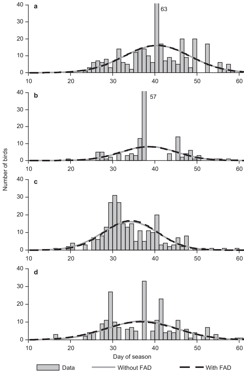
Fig. 3. Number of observed tree pipits at the Hanko Bird Observatory (grey bars), for the years (a) 2006, (b) 2007, (c) 2008 and (d) 2009. A Gaussian functions fitted without FAD and with FAD included as data are shown as grey solid and black dashed lines, respectively.
