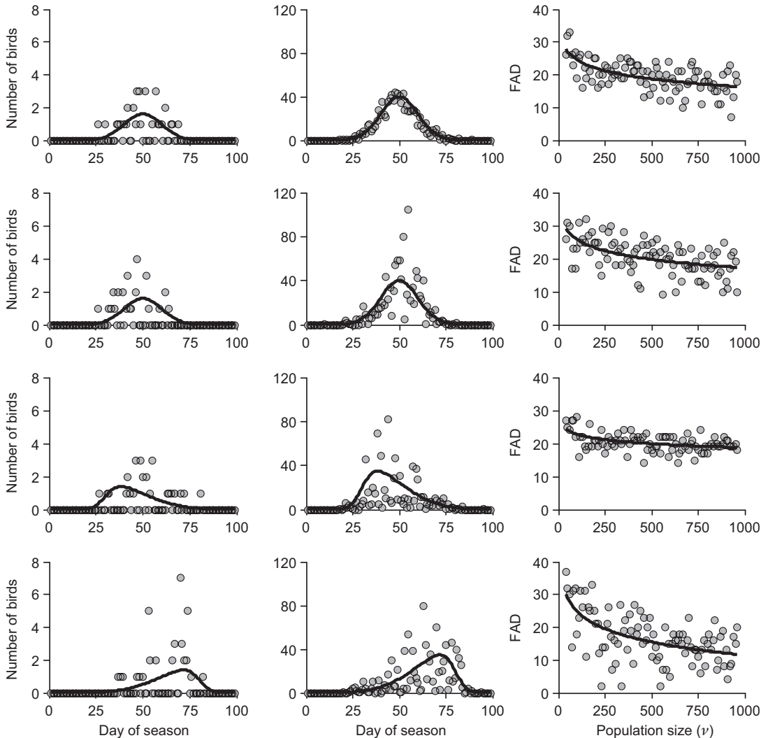
Fig. 1. Simulated scenarios of counted migration numbers with expected population size (parameter \nu ) 40 individuals (left-hand-side column of figure panels), 960 individuals (middle column), and the fitted log-normal relationships between FAD and population size when the phenological distributions are kept constant (right-hand-side column). The rows of panels, from top downwards, represent scenarios with different parameter values (Table 1): (i) Gaussian distribution with the Poisson error, (ii) Gaussian distribution with the neg. bin. error, (iii) right-skewed function with the neg. bin. error, and (iv) left-skewed function with the neg. bin. error.
