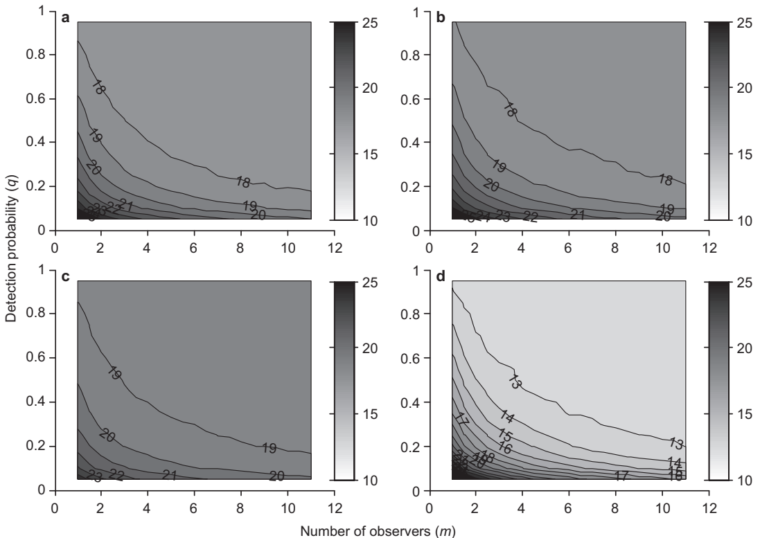
Fig. 2. Average FAD under the four investigated scenarios (a–d) with varying number of observers ( m ; x-axis) and detection probability ( q ; y-axis). Population size ( \nu ) is fixed to 1000. The average FAD is illustrated both as shades of grey and with contour lines.
