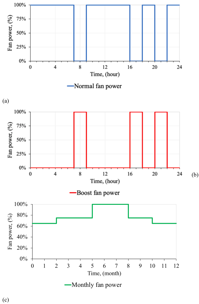
Fig. 2. Hourly normal and boost fan power (a and b) and monthly fan power (c) profiles in the reference building model.
