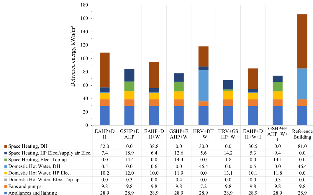
Fig. 7. The delivered energy use in different renovation packages.
