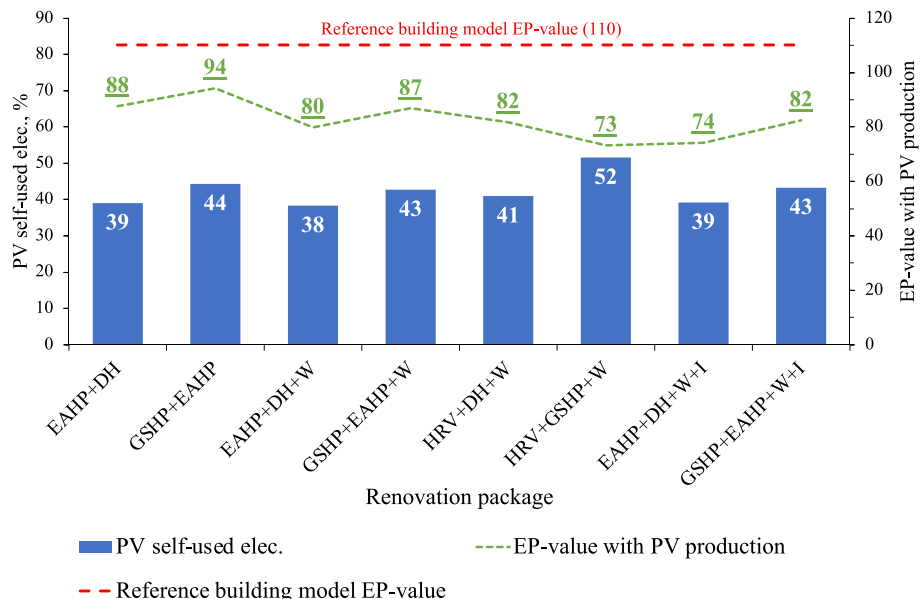
Fig. 11. The PV self-used electricity and calculated EP-value considering PV elec. production between different renovation packages.
