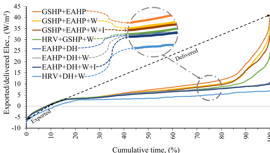
Fig. 12. The exported/delivered electricity unit load in different renovation packages considering PV production electricity.
