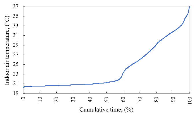
Fig. 5. The indoor air temperature duration curve of the coldest apartment in the reference building model.
