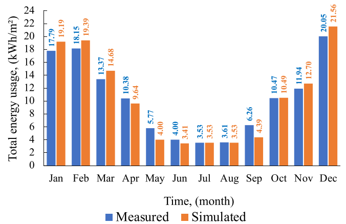
Fig. 4. The measured vs calibrated simulated total energy usage in building 4.
