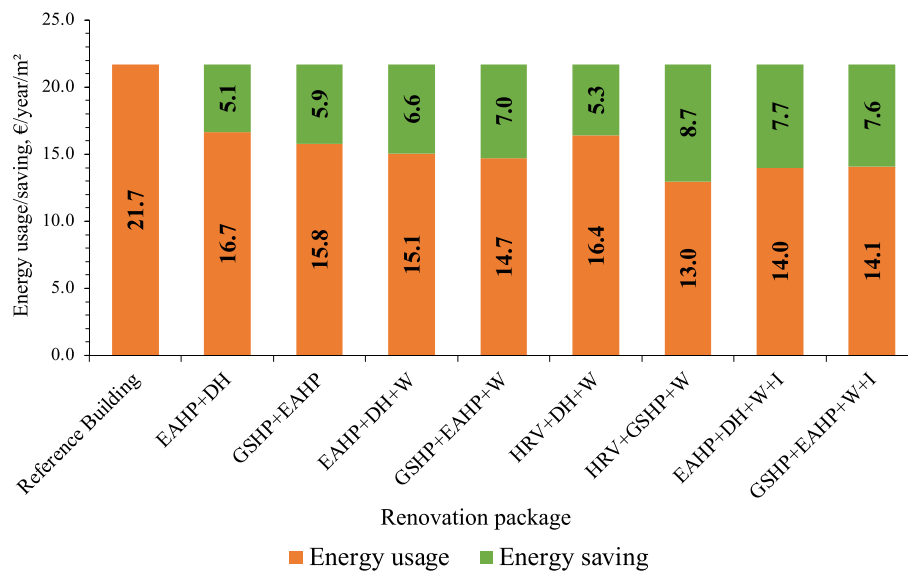
Fig. 13. The annual energy cost including both electricity and district heat and saving in different renovation packages.
