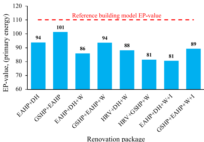
Fig. 8. The EP-value of renovation packages.
