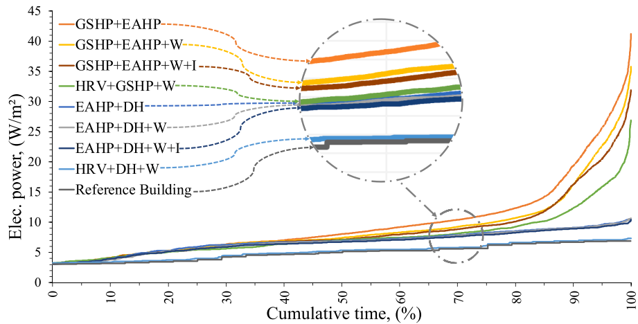
Fig. 10. The electricity power specific consumption duration curve in renovation packages.
