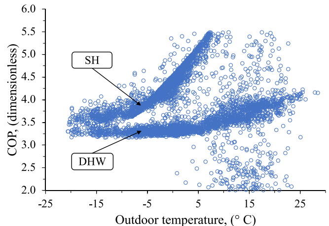
Fig. 9. The Coefficient of Performance (COP) as a function of outdoor temperature in the EAHP renovation package.
