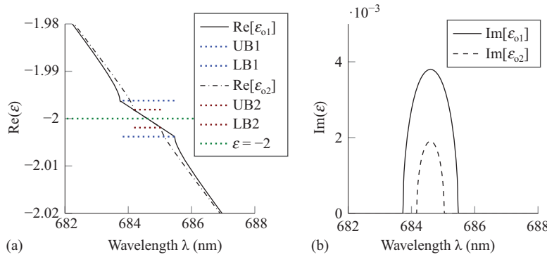
Figure 20.6 Real and imaginary parts of the optimized permittivity functions approximating a metamaterial with \varepsilon_t = -2 . Here, \varepsilon_{01} and \varepsilon_{02} are optimized using (20.58) and linear B-splines, for the relative bandwidths B = 2.5 \cdot 10^{-3} and B = 1.25 \cdot 10^{-3} , respectively. UB1-2 and LB1-2 denote the corresponding upper and lower physical bounds based on (20.45)
