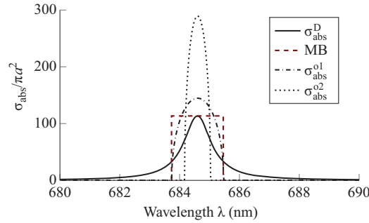
Figure 20.5 Absorption cross section \sigma_{\text{abs}}^{\text{D}} of a small ( a = 5 nm) gold nanosphere modeled by using a dielectric Drude model. The red dashed line (MB) gives the maximal bandwidth for the corresponding peak resonance based on the associated sum rule \Delta\lambda = 4\pi^3 a^3 / \max \sigma_{\text{abs}}^{\text{D}} . Here, \sigma_{\text{abs}}^{\text{01}} and \sigma_{\text{abs}}^{\text{02}} correspond to optimized permittivity functions for relative bandwidths B = 2.5 \cdot 10^{-3} and B = 1.25 \cdot 10^{-3} , respectively
