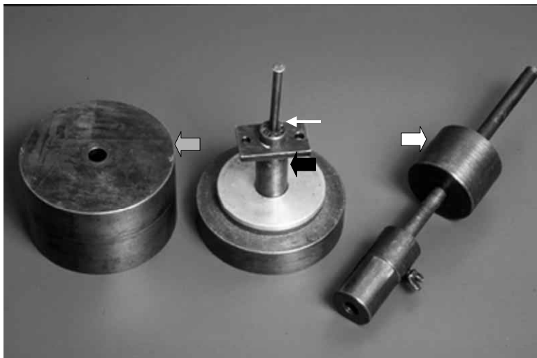
Figure 18: Miniature impactor - grafting material is placed in a 15-mm-diameter impaction chamber (black arrow). A perforated piston (small white arrow) allows elimination of air and fluid during impaction. The impactor and piston are enclosed within a chamber (left grey block arrow) to improve stability. A brass cylinder (right white arrow) is dropped over the piston, to produce a compaction level similar to that generated during revision hip arthroplasty
