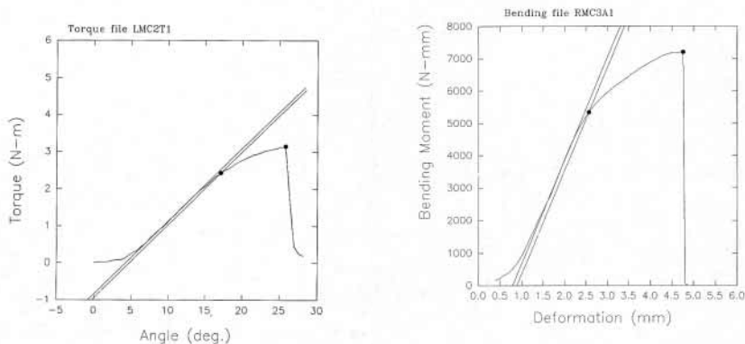
Figure 28: Load deformation curves.
