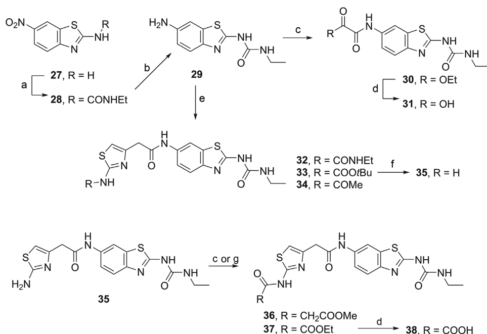
SCHEME 3 Synthesis of compounds 28–38. Reagents and conditions. a) Ethyl isocyanate, \text{Et}_3\text{N} , toluene, reflux, 24 h. b) \text{H}_2 , Pd/C, \text{EtOH}/\text{DMF} , r.t., 48 h. c) Ethyl oxalyl chloride, \text{Et}_3\text{N} , 1,4-dioxane, r.t., 18 h. d) 1 M NaOH, \text{MeOH}/\text{H}_2\text{O} , r.t., 18 h. e) Carboxylic acid, EDC, HOBT, NMM, DMF, r.t., 18 h. f) Acetyl chloride, \text{MeOH} , 0^\circ\text{C} , 1 h, then r.t., 18 h. g) Methyl malonyl chloride, \text{Et}_3\text{N} , 1,4-dioxane, r.t., 18 h
