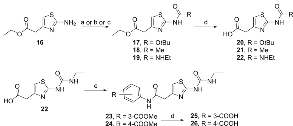
SCHEME 2 Synthesis of compounds 17–26. Reagents and conditions: a) 17: \text{Boc}_2\text{O} , 4-dimethylaminopyridine, \text{CH}_2\text{Cl}_2 , r.t., 18 h. b) 18: Acetyl chloride, \text{Et}_3\text{N} , \text{CH}_2\text{Cl}_2 , r.t., 4 h. c) 19: Ethyl isocyanate, \text{CHCl}_3 , 50^\circ\text{C} , 18 h. d) 2 M NaOH, \text{MeOH}/\text{H}_2\text{O} , r.t., 18 h. e) Amine, EDC, HOBT, NMM, DMF, r.t., 24 h
