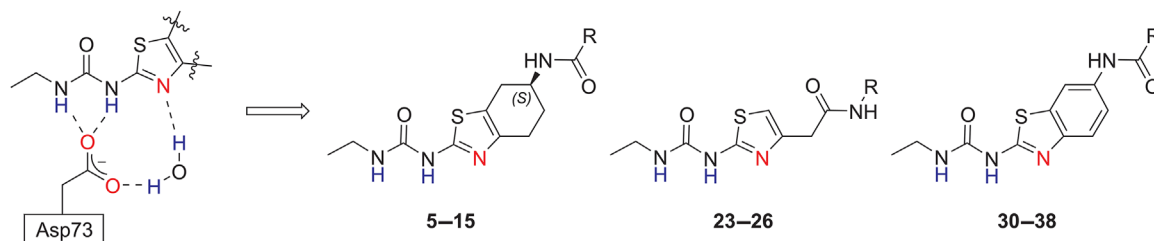
FIGURE 2 The hydrogen bonds of the thiazole-based ethylureas in the ATP binding site of DNA gyrase ( E. coli numbering) and designed novel thiazole-based ethylurea DNA gyrase B inhibitors
