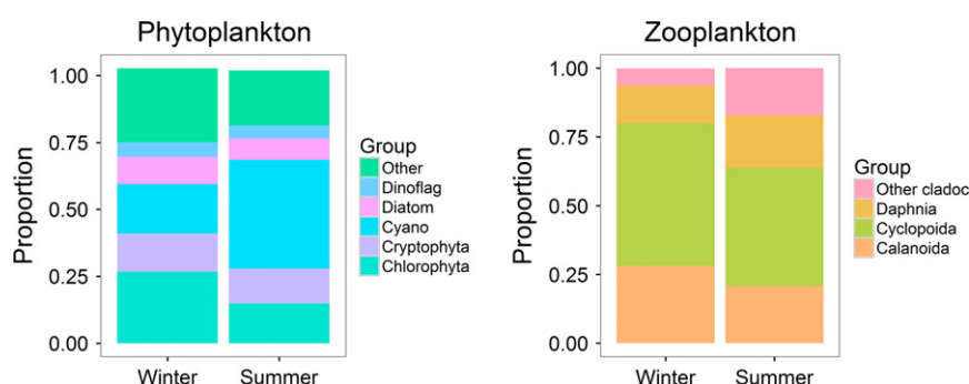
Figure 3 Average community composition for major phytoplankton and crustacean zooplankton groups during the winter and summer seasons, expressed as a proportion of total density.
