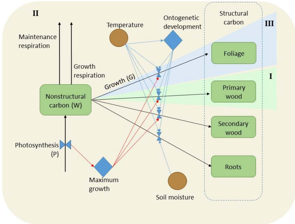
Figure 5. Model structure. State variables are shown in green rectangles and carbon flows are depicted by black arrows. Environmental factors are depicted by brown circles and inherent variables by blue diamonds. The red and blue arrows indicate source and sink effect, respectively. Coloured areas with roman numbers refer to contents studied in papers I, II and III.
