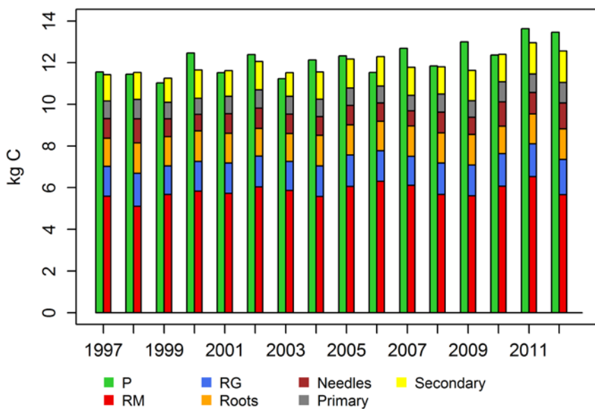
Figure 9. The components of carbon balance (II). Photosynthesis (P) is a source of carbon whereas RM (maintenance respiration), RG (growth respiration) and the growing organs are carbon sinks.
