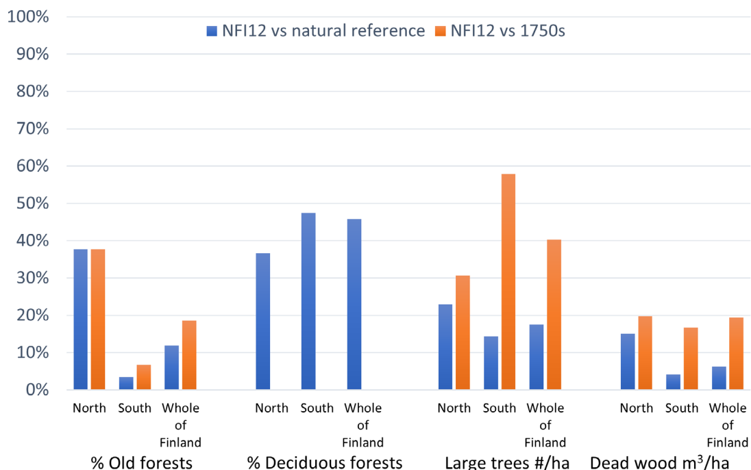
Figure 1. Percentage cover of old forests and deciduous forests, density of large trees and dead wood volumes in Finland according to NFI12 relative to values under natural reference conditions (blue bars) and in the 1750s (orange bars). The values are given for North (northern boreal forests), South (middle- & south- & hemiboreal forests), and for whole Finland.
