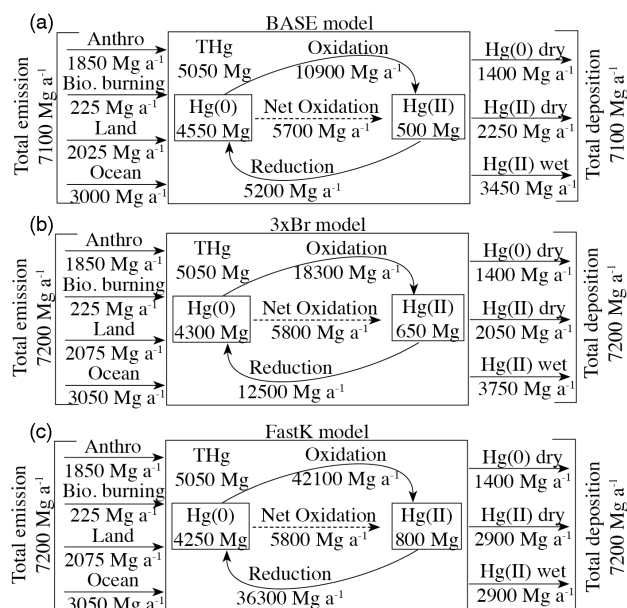
Figure 9. Annual global tropospheric budget of mercury in the (a) BASE, (b) 3\times Br, and (c) FastK simulations for 2013. The burdens are in units of Mg ( 10^6 g) and the fluxes are in units of \text{Mg a}^{-1} ( \text{Mg} per year).
